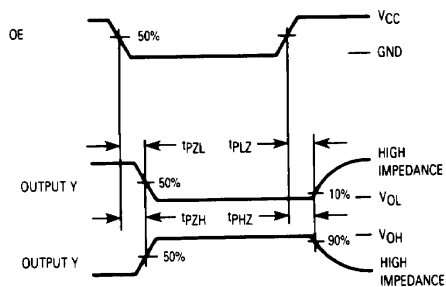
Figure 2. Switching Waveforms
