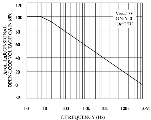
Figure 2. Open-Loop Frequency
