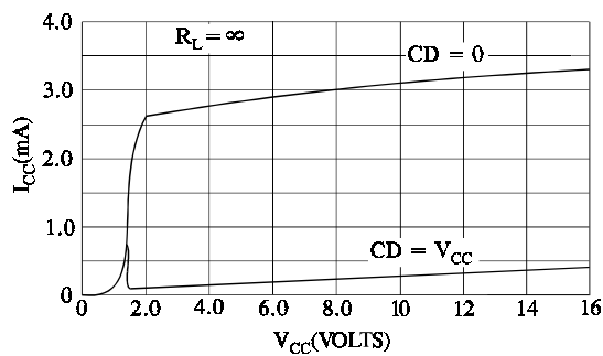
Figure 1. POWER SUPPLY CURRENT
