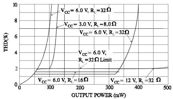
Figure 6. DISTORTION versus POWER f = 3.0 kHz, AVD = 34 dB
