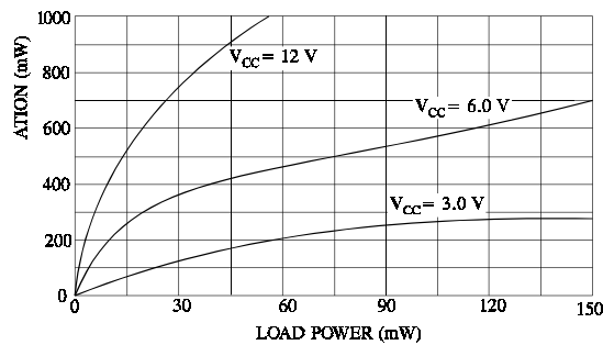
Figure 2. DEVICE DISSIPATION 8.0 \Omega LOAD
