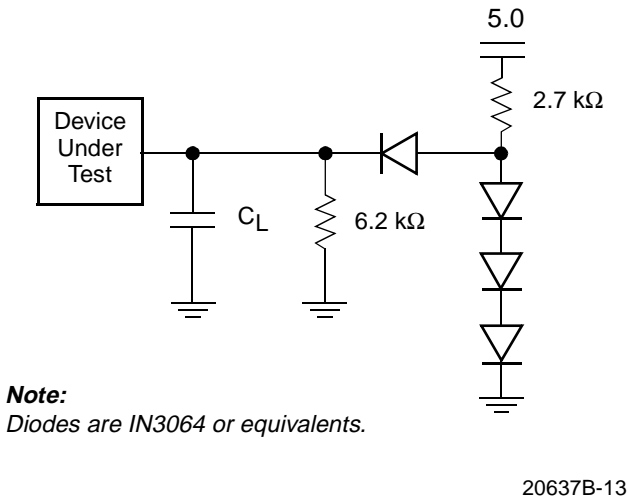
Figure 8. Test Setup
