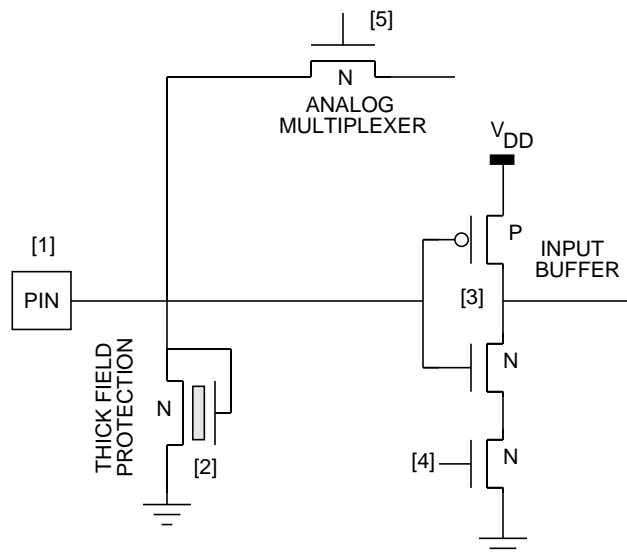
Figure 2-16 Internal Circuitry — Analog Input-Only Pin
