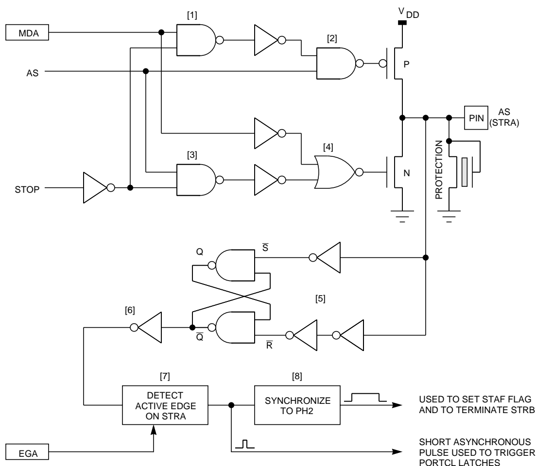
Figure 7-15 AS (STRA) Pin Logic
