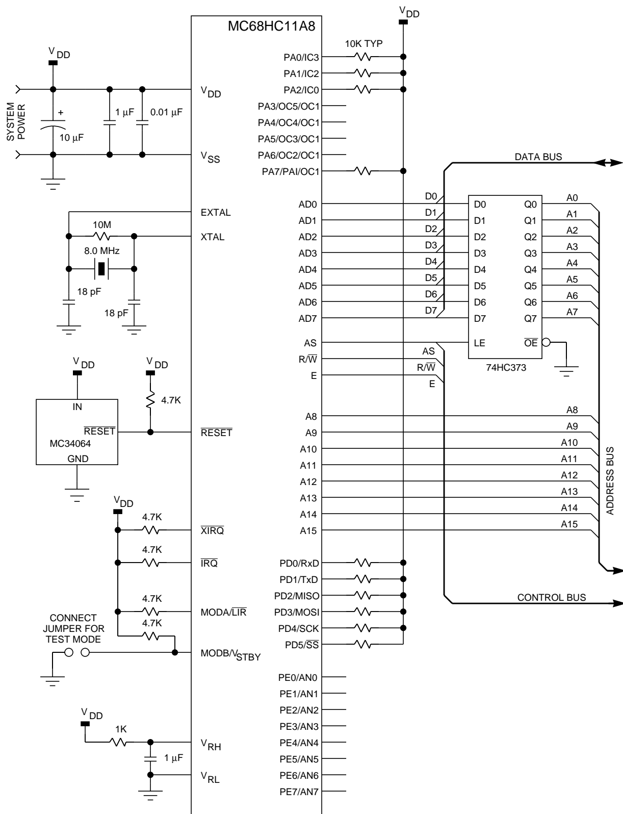
Figure 2-23 Basic Expanded Mode Connections (Sheet 1 of 2)
