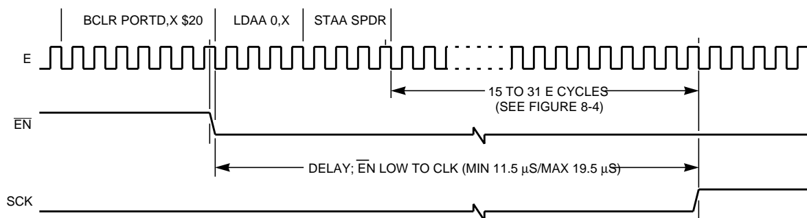
a) \overline{EN} low to clock start delay (MC144110 needs 5 μS)
