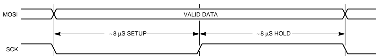
b) Data valid vs. clock timing (MC144110 needs 1 μS setup/ 5 μS hold)
