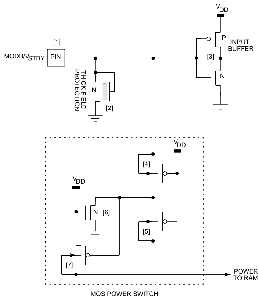
Figure 2-20 Internal Circuitry — MODB/V STBY Pin
