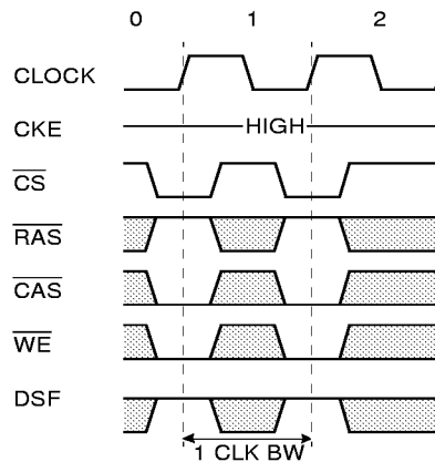
Timing Diagram to Illustrate tbwc
