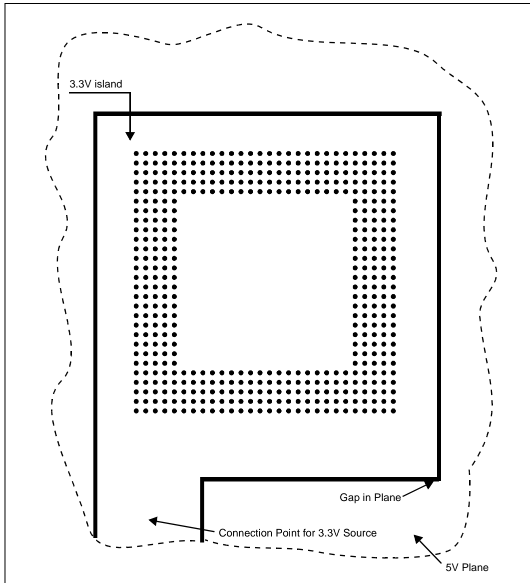
Figure 9-17. Creating a Power “Island”
