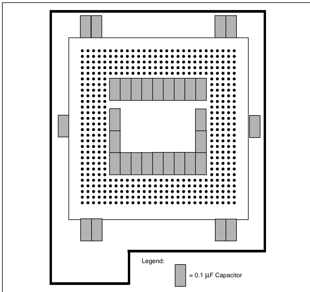
Figure 10-23. High-Frequency Capacitor Values and Layout
