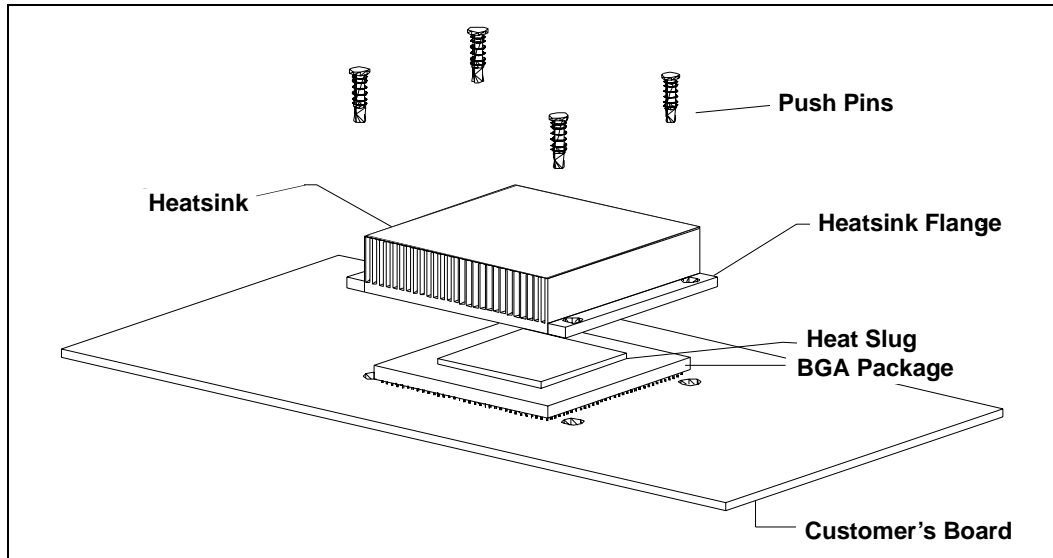
Figure 14-32. Conceptual 3-D View of Processor with a Heat Sink
