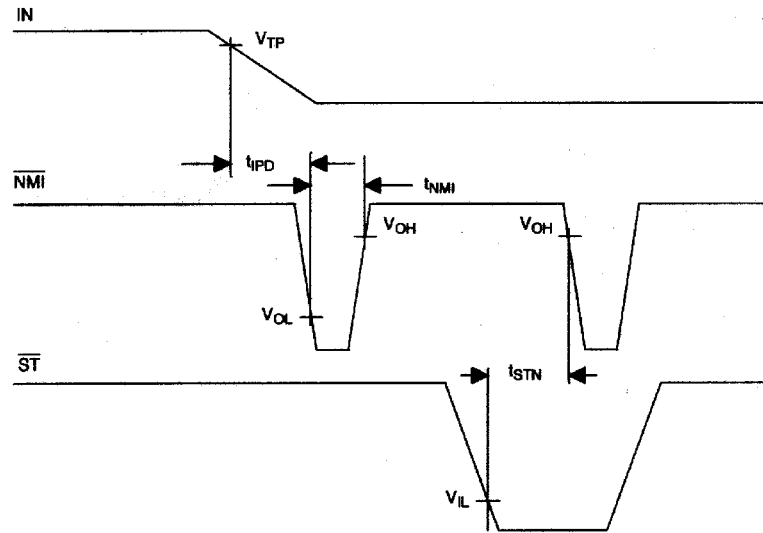
POWER MONITOR, WATCHDOG Figure 4
