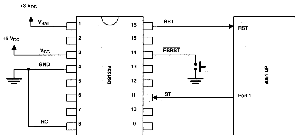
POWER MONITOR, WATCHDOG Figure 4
