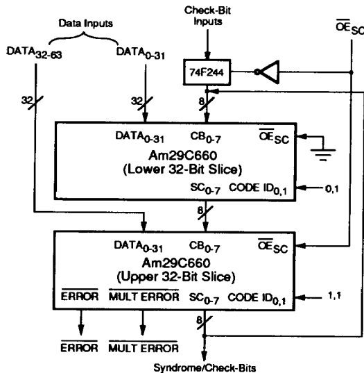
Figure 8. 64-Bit Configuration
