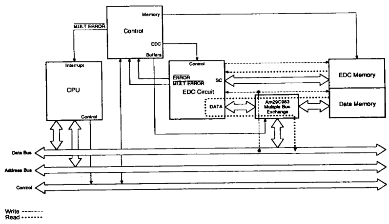
Figure 10. Correct-Always Configuration
