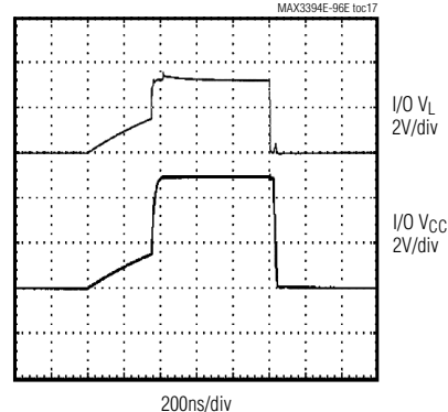
(DRIVING I/O V_L , V_{CC} = +5.0\text{V} , V_L = +3.3\text{V} , C_L = 400\text{pF} , EXTERNAL 4.7\text{k}\Omega PULLUPS, DATA RATE = 1Mbps)
