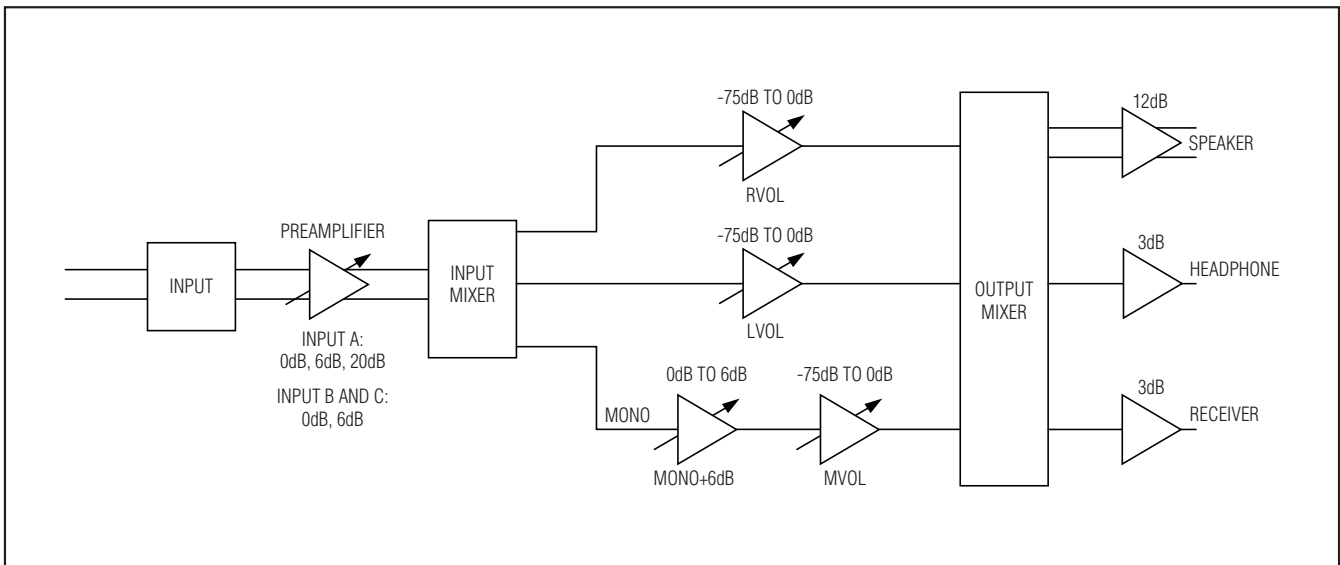
Figure 7. Signal Path
