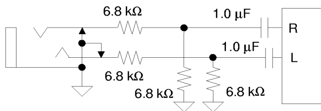
Figure 26. Line Inputs
