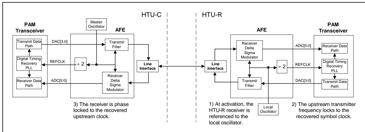
Figure 18. Clock Generation
