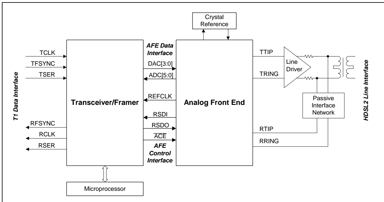
Figure 4. HDSL2 Modem
