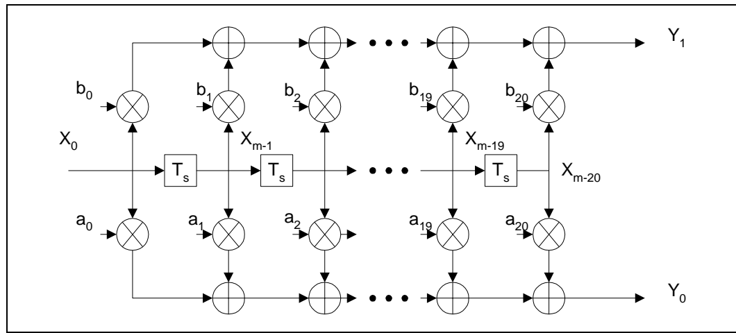
Figure 15. Convolutional Encoder
