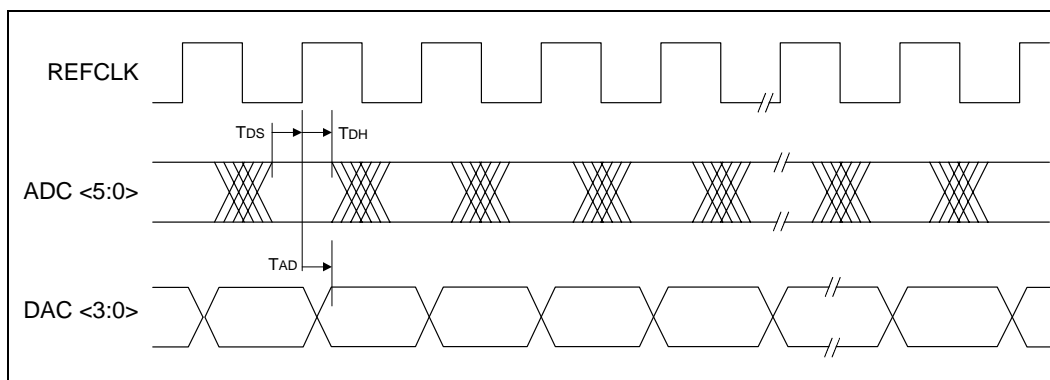
Figure 24. AFE Data Interface Relative Timing
