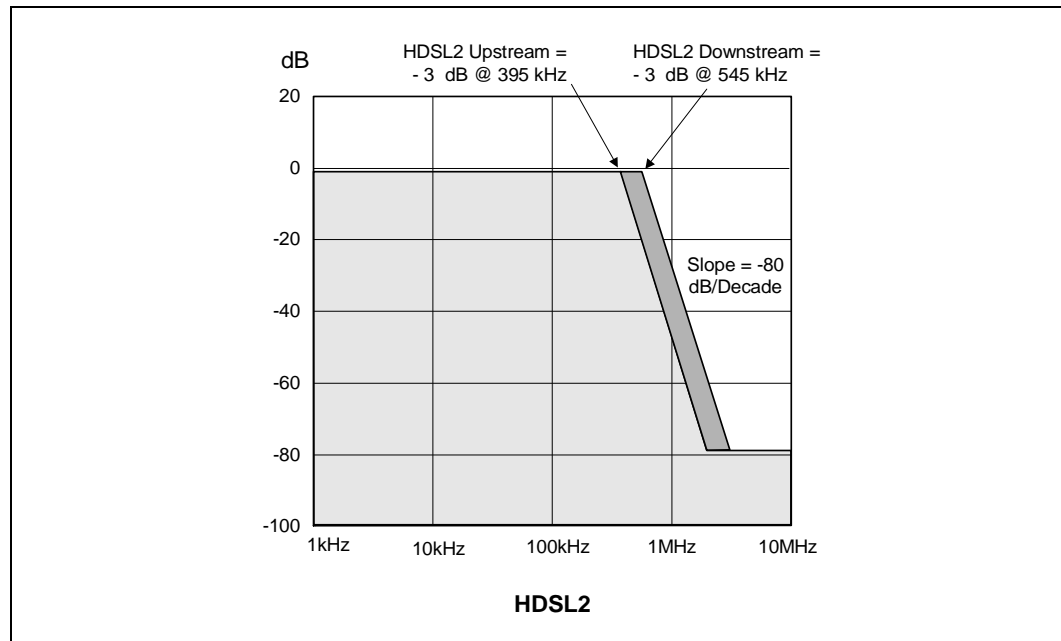
Figure 6. Transmit Frequency Response
