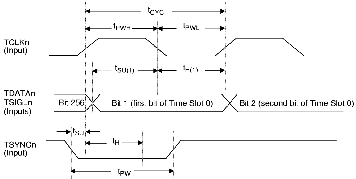
Figure 20. Transmit Highway Timing - 2 Mbit/s MVIP Mode
