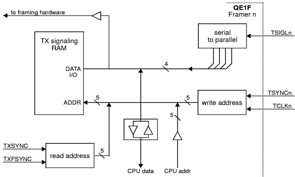
Figure 51. Transmit Signaling Buffer
