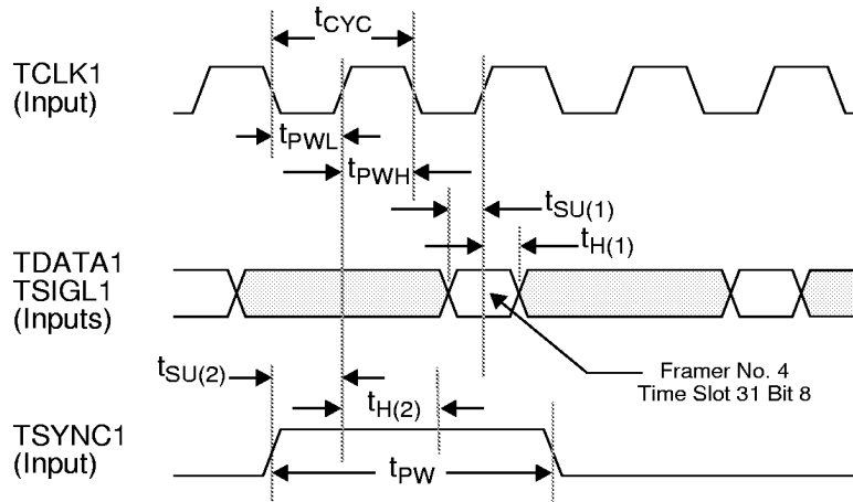
Figure 15. Transmit Highway Timing - 8 Mbit/s Transmission Mode
