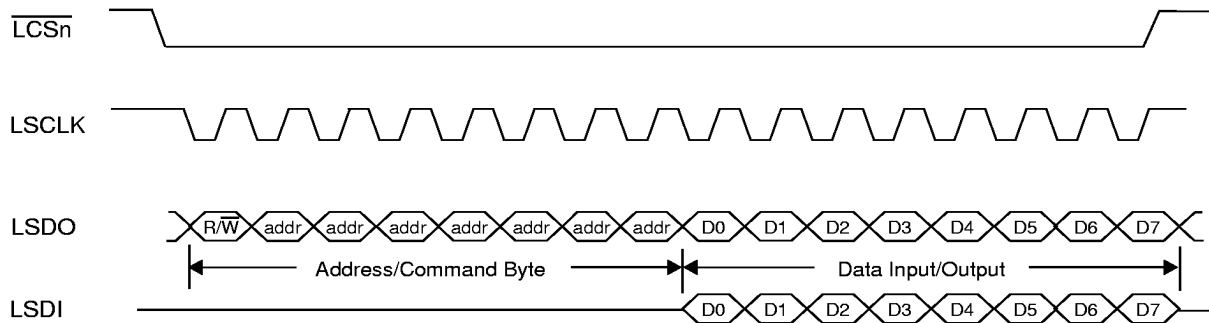
Figure 33. Transceiver Serial I/O Timing
