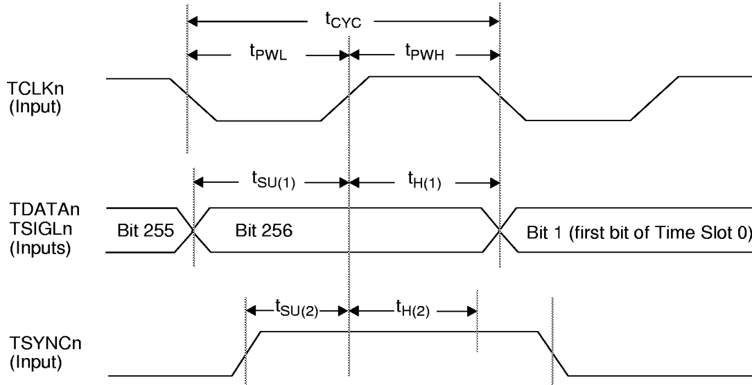
Figure 18. Transmit Highway Timing - 2 Mbit/s Transmission Mode
