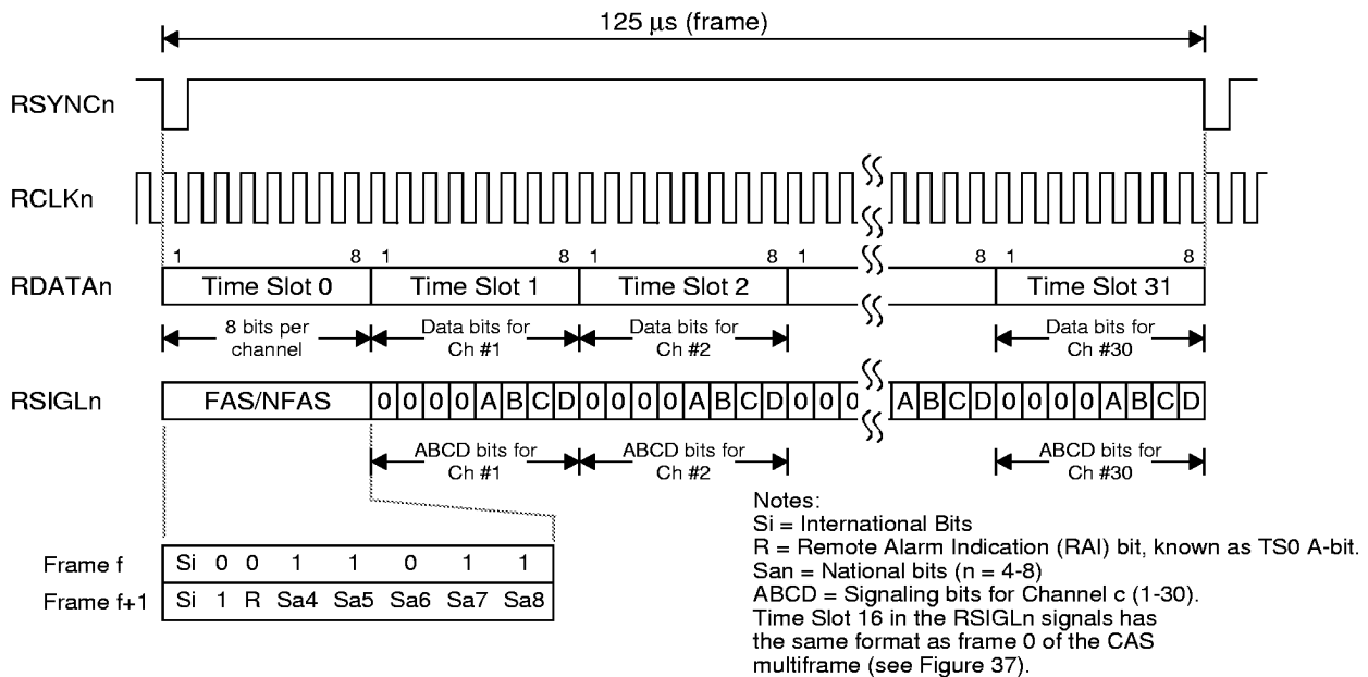
Figure 43. Receive Highway - 2 Mbit/s MVIP Mode
