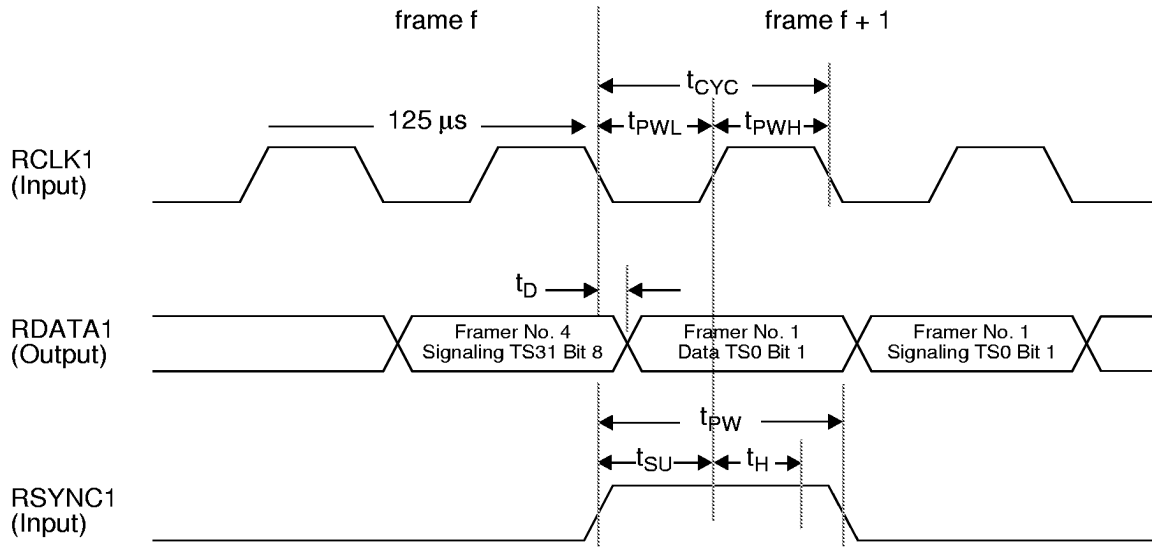
Figure 23. Receive Highway Timing - 16 Mbit/s PCM Highway Mode
