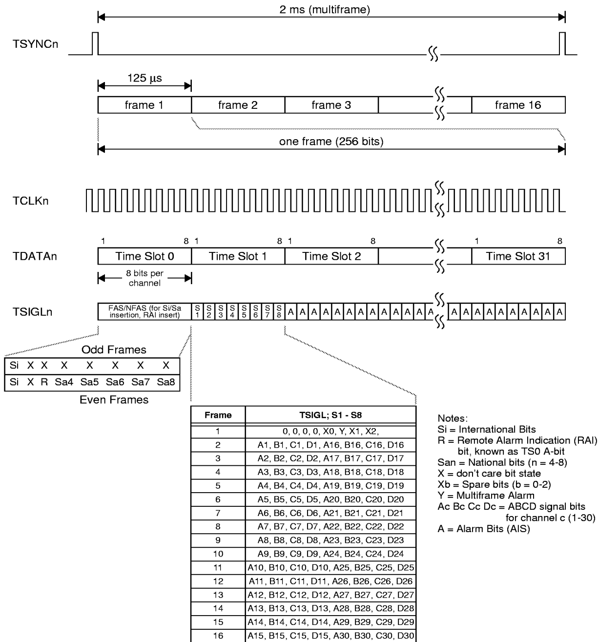
Figure 36. Transmit Highway - 2 Mbit/s Transmission Mode
