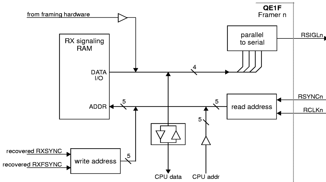
Figure 50. Receive Signaling Buffer
