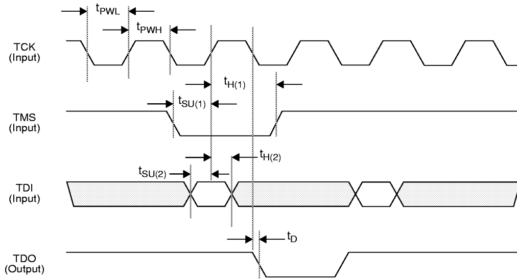
Figure 26. Boundary Scan Timing
