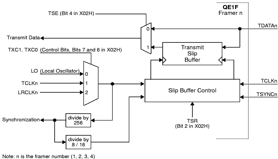
Figure 48. Transmit Slip Buffer
