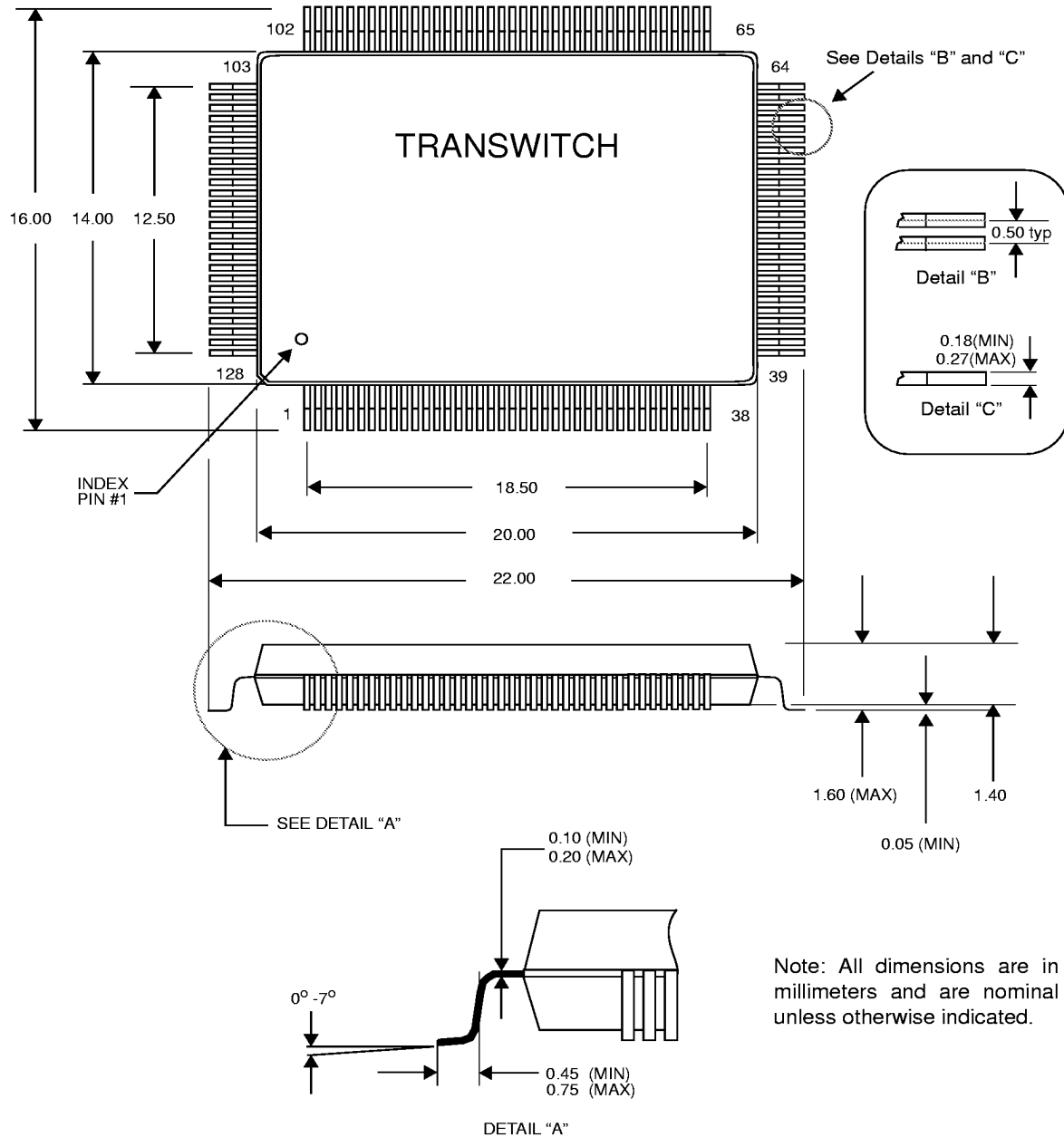
Figure 57. QE1F TXC-03104 128-Pin Thin Plastic Quad Flat Package
