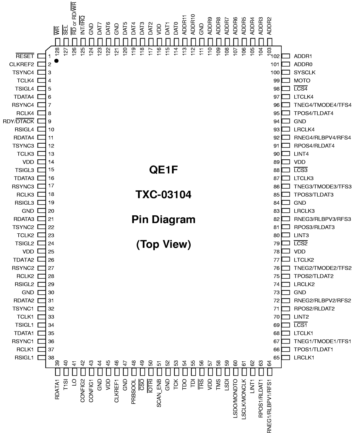
Figure 2. QE1F TXC-03104 Pin Diagram
