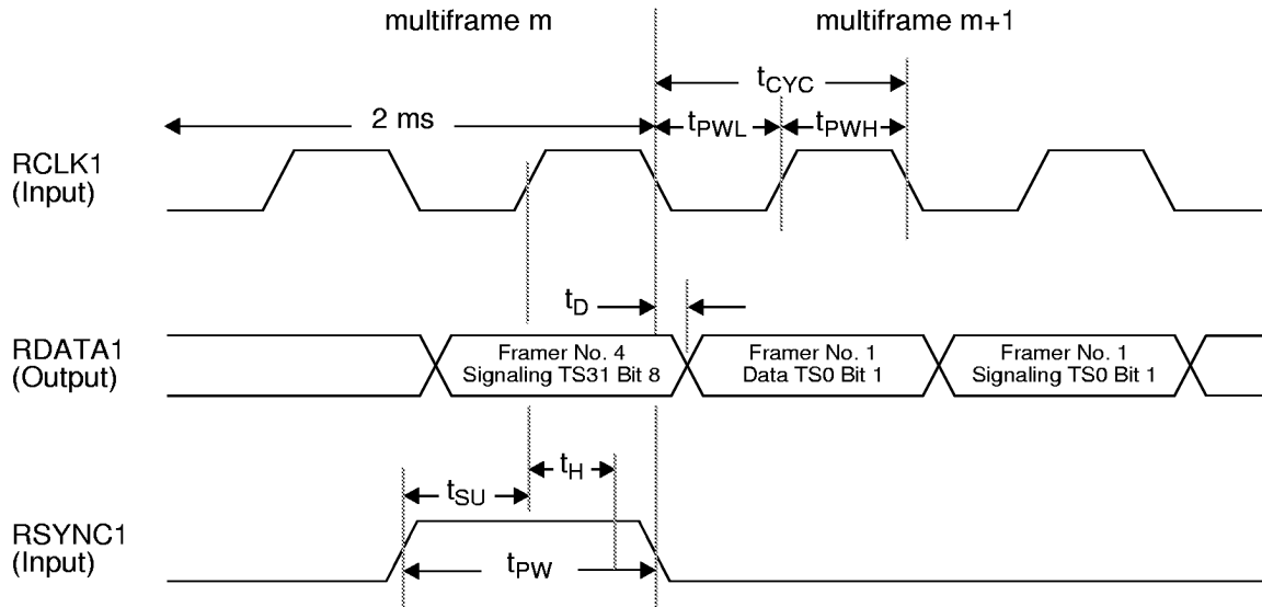
Figure 16. Receive Highway Timing - 16 Mbit/s Transmission Mode
