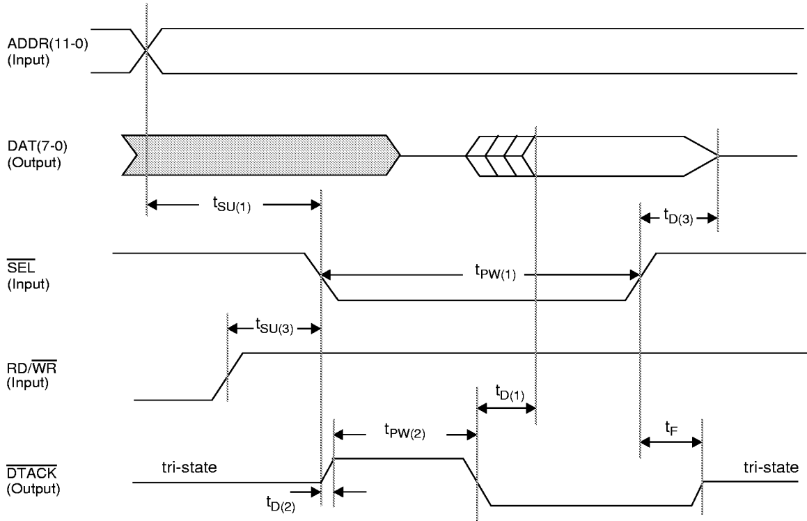
Figure 29. Motorola Microprocessor Read Cycle Timing
