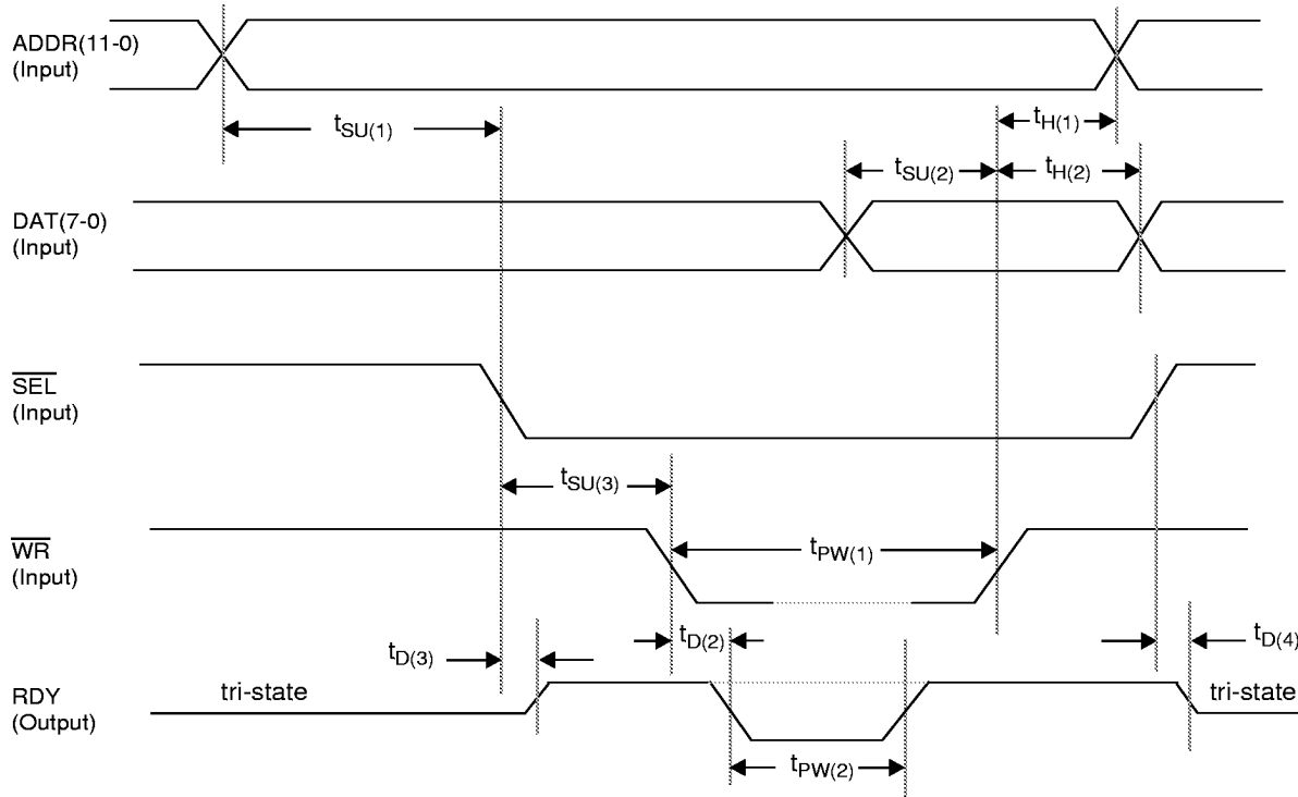
Figure 28. Intel Microprocessor Write Cycle Timing
