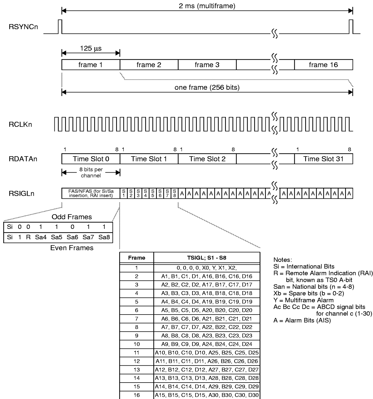
Figure 37. Receive Highway - 2 Mbit/s Transmission Mode
