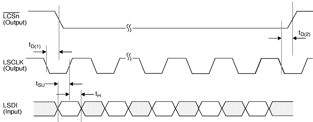
Figure 10. Serial Port Read Timing
