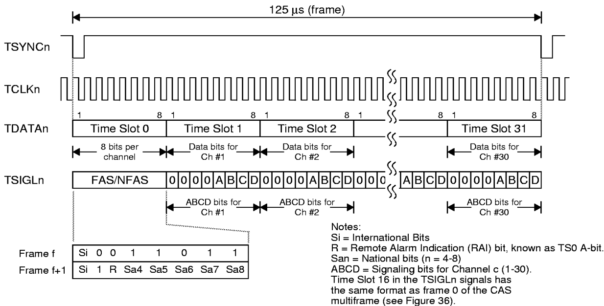
Figure 42. Transmit Highway - 2 Mbit/s MVIP Mode
