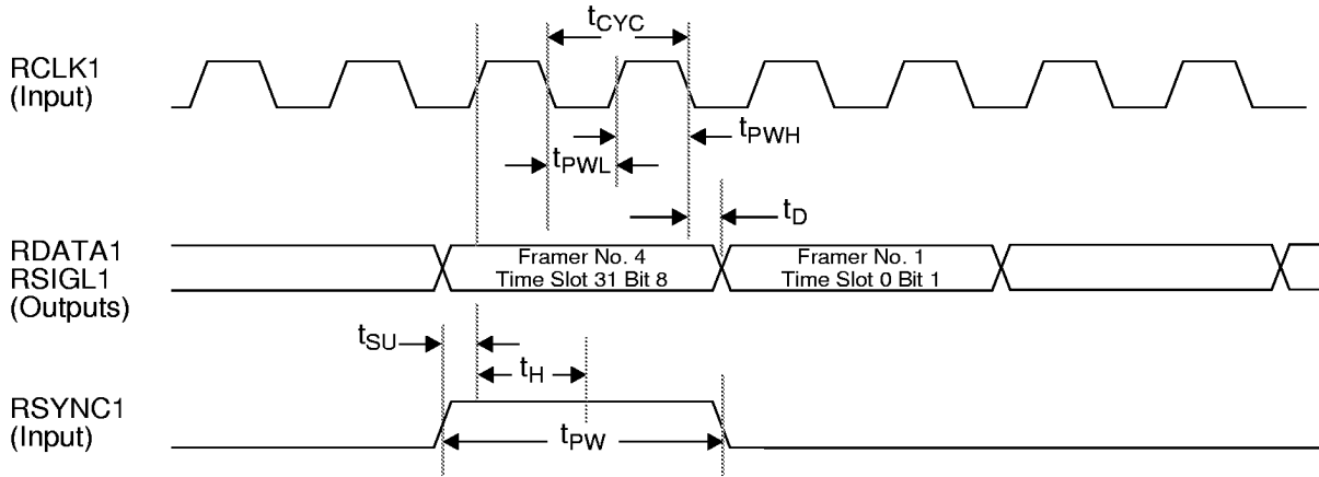
Figure 14. Receive Highway Timing - 8 Mbit/s Transmission Mode
