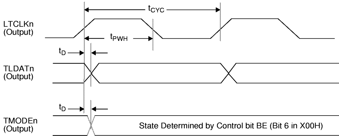
Figure 6. NRZ Transmit Interface Timing (External Transceiver)
