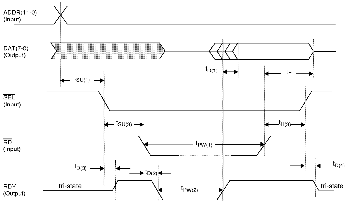
Figure 27. Intel Microprocessor Read Cycle Timing
