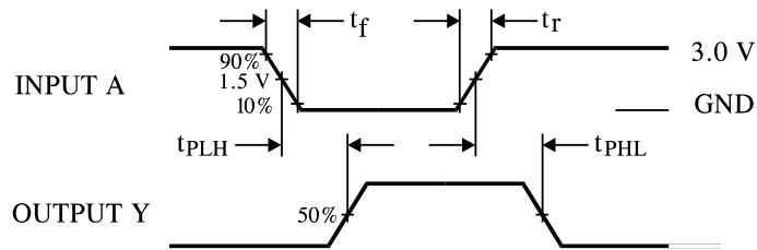
Figure 1. Switching Waveforms
