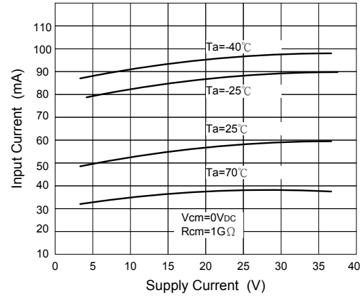
Fig.2 Input Current
