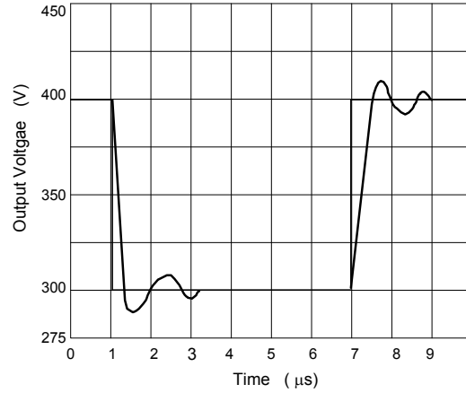
Fig.7 Voltage Follower Pulse Response (Small Signal)
