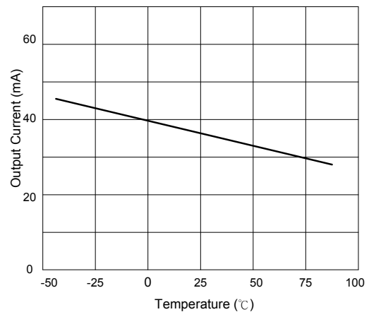
Fig.11 Current Limiting
