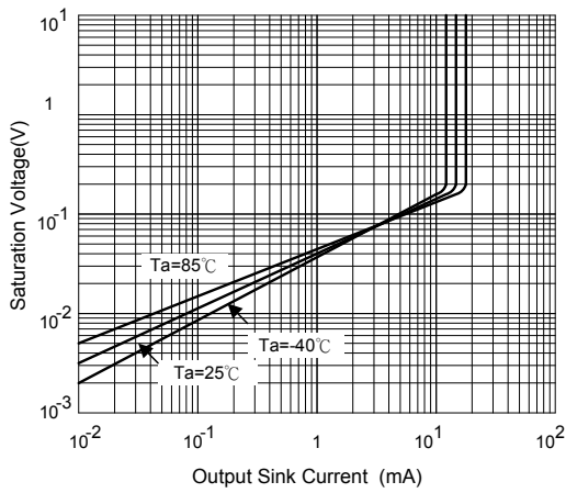
Fig.3 Output Saturation Voltage
