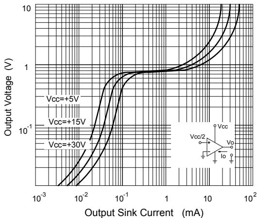
Fig.10 Output Characteristics Current Sinking
