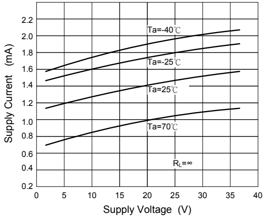
Fig.1 Supply Current
