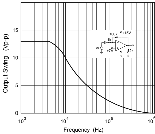
Fig.8 Large Signal Frequency Response
