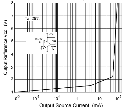
Fig.9 Output Characteristics Current Sourcing
