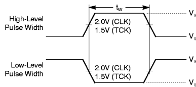
Figure 16. Voltage Waveforms - Clock Pulse Duration
