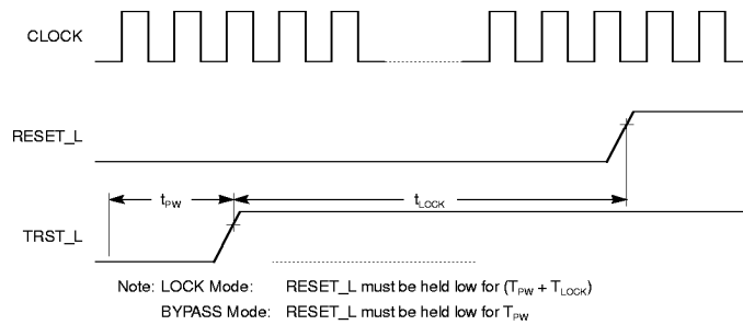
Figure 18. Reset Timing
