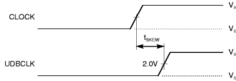
Figure 17. Voltage Waveforms - Clock Skew
