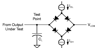
Figure 13. Load Circuit
