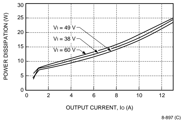
Figure 22. FE150B Power Dissipation as Heat vs. Output Current
