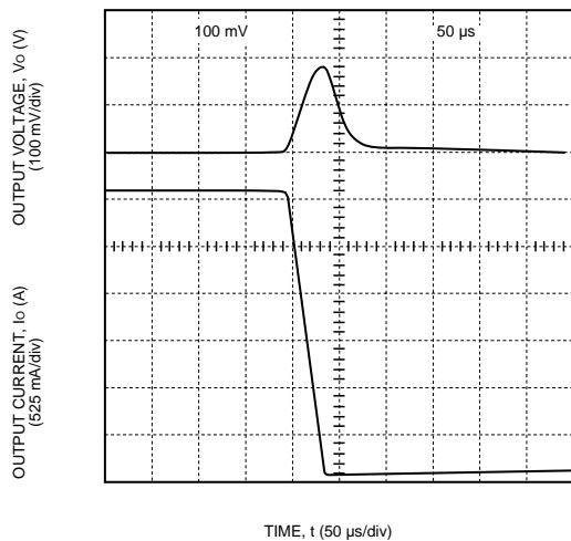
Figure 6. Typical FE150B Transient Response to Step Decrease in Load from 50% to 25% of Full Load at Room Temperature and 48 V Input (Waveform Averaged to Eliminate Ripple Component.)
