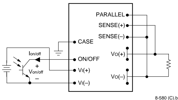
Figure 12. Remote On/Off Implementation
