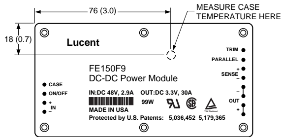
Note: Top view, measurements shown in millimeters and (inches). 8-582 (C),r
