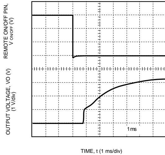
Figure 7. Typical FE150F Start-Up Transient at Room Temperature, 48 V Input, and 30 A Output
