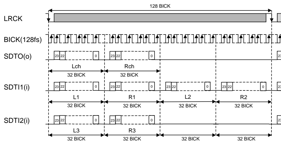
Figure 12. Mode 11 Timing
