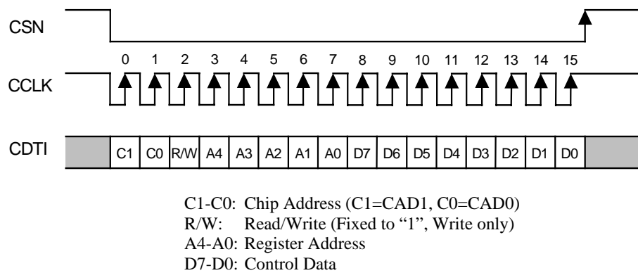
Figure 16. 3-wire Serial Control I/F Timing
