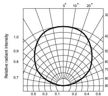
Fig.6 Radiation diagram
