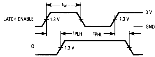
Figure 2. Switching Waveforms
