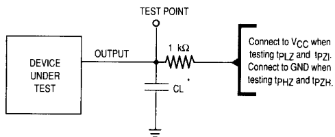
Figure 6. Test Circuit
