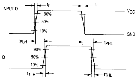
Figure 1. Switching Waveforms
