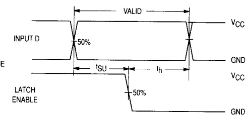
Figure 2. Switching Waveforms
