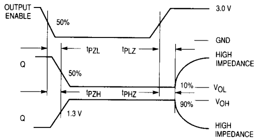
Figure 3. Switching Waveforms
