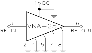
TYPICAL BIASING CONFIGURATION
