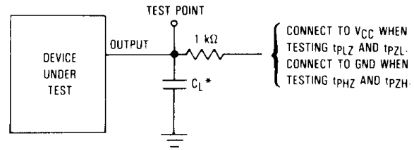
Figure 4. Test Circuit
