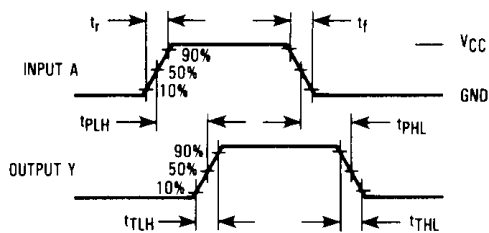
Figure 1. Switching Waveforms
