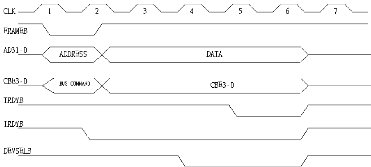
Figure 7. Target Write
