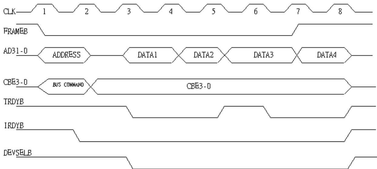
Figure 11. Memory Read
