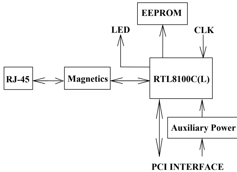
Figure 18. Application Information
