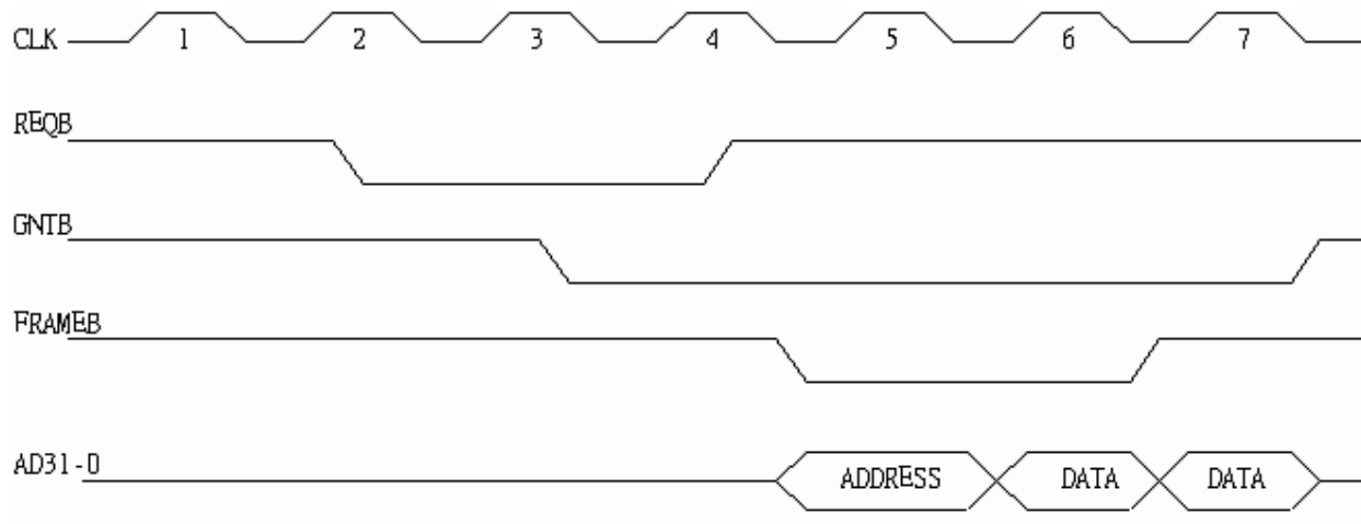
Figure 10. Bus Arbitration
