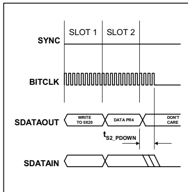
Figure 20 AC-Link Powerdown Timing
