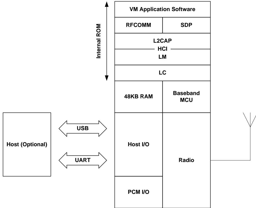
Figure 8.3: Virtual Machine
