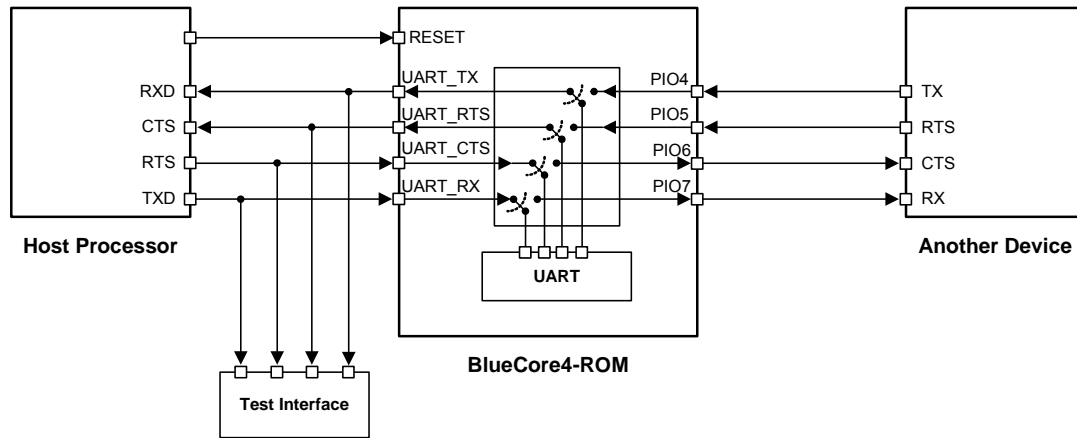
Figure 10.13: UART Bypass Architecture
