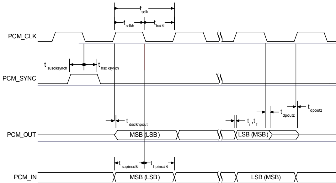
Figure 10.29: PCM Slave Timing Short Frame Sync
