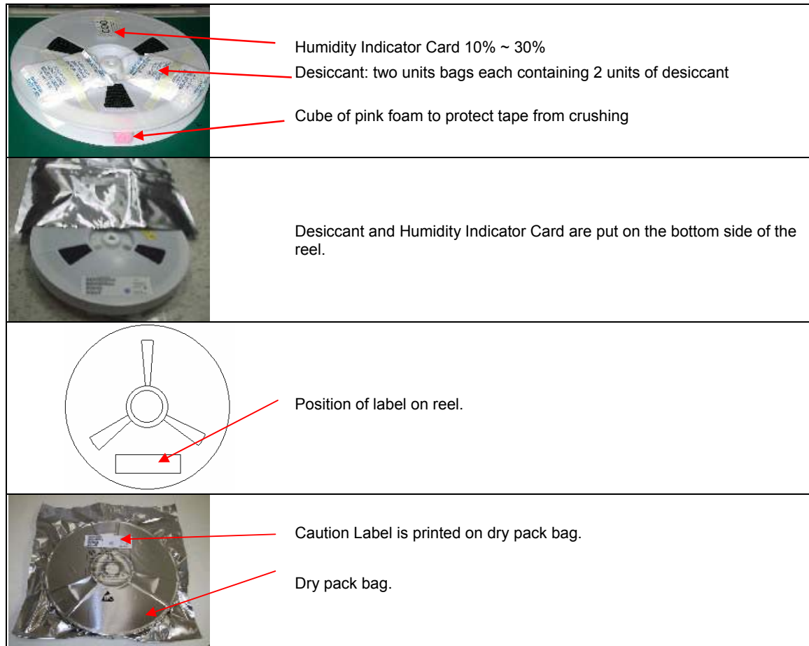
Figure 15.4: Tape and Reel Packaging
