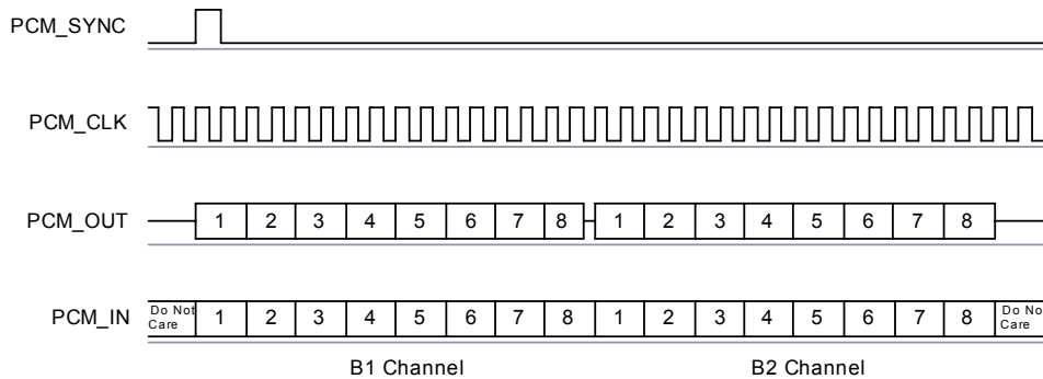
Figure 10.24: GCI Interface
