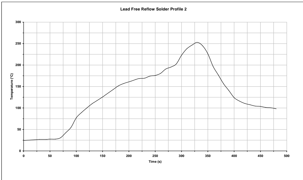
Figure 13.1: Typical Lead-Free Re-flow Solder Profile
