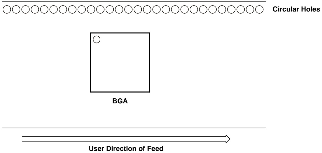
Figure 15.1: Tape and Reel Orientation
