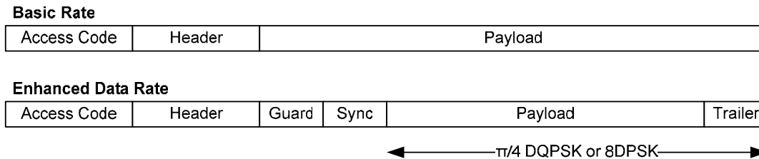
Figure 9.1: Basic Data Rate and Enhanced Data Rate Packet Structure
