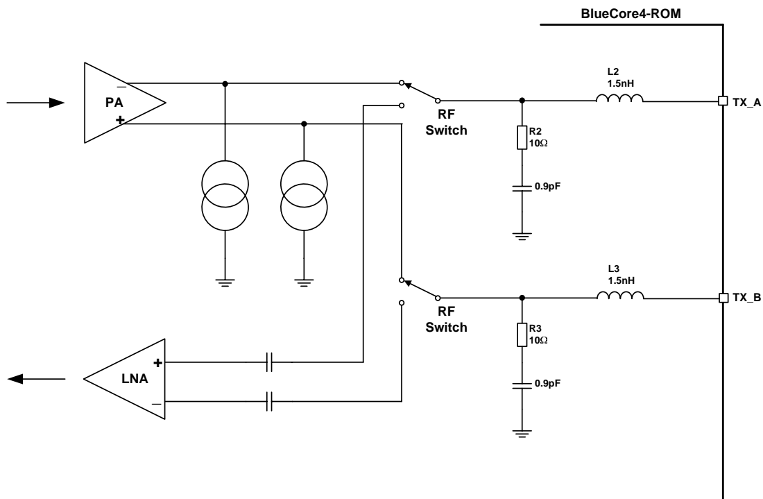
Figure 10.1: Circuit TX/RX_A and TX/RX_B
