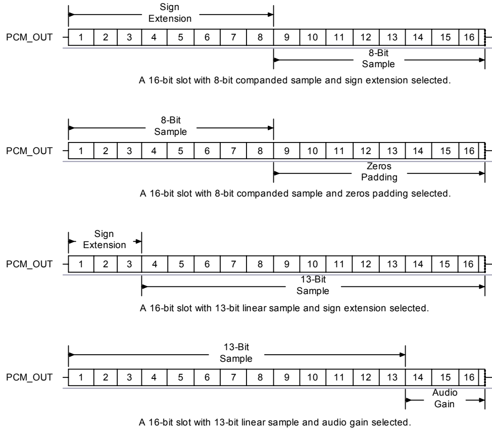
Figure 10.25: 16-Bit Slot Length and Sample Formats
