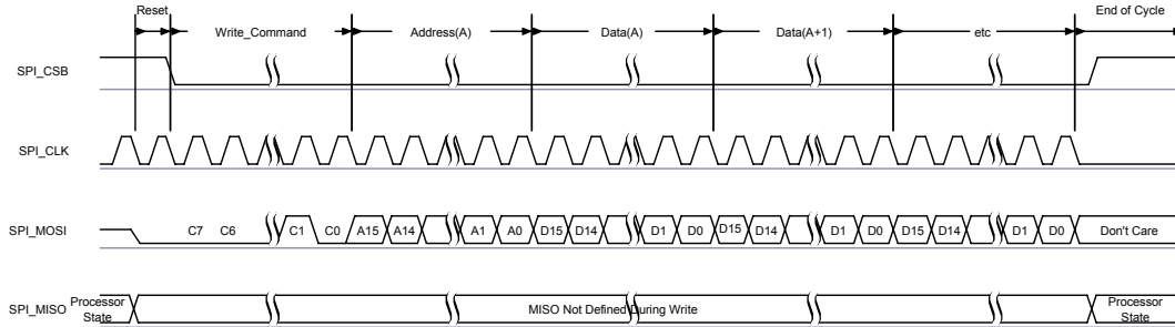
Figure 10.17: Write Operation
