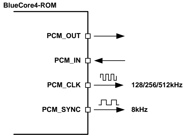
Figure 10.19: BlueCore4-ROM as PCM Interface Master
