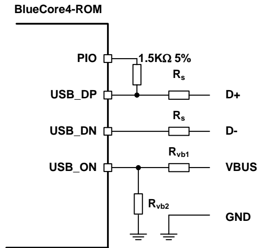
Figure 10.14: USB Connections for Self Powered Mode
