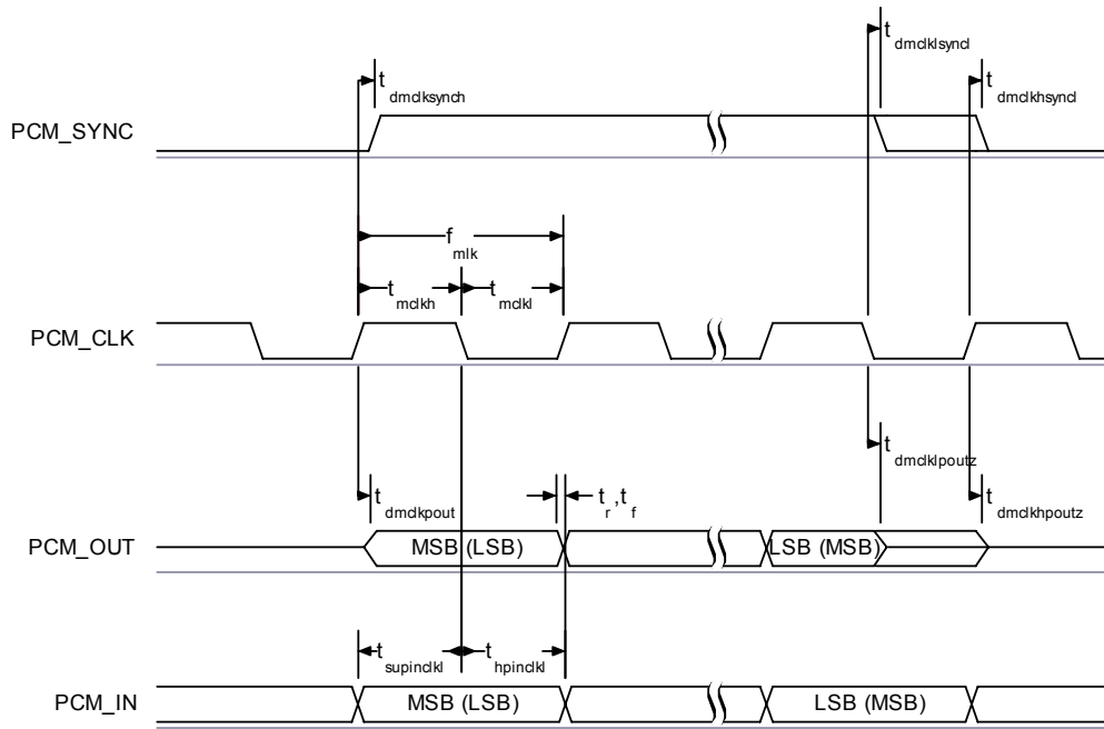
Figure 10.26: PCM Master Timing Long Frame Sync
