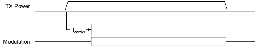
Figure 10.3: Internal Power Ramping
