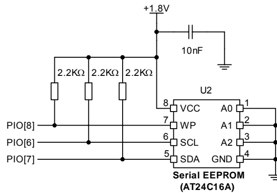
Figure 10.30: Example EEPROM Connection
