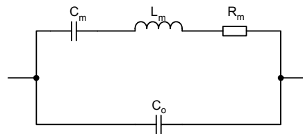
Figure 10.7: Crystal Equivalent Circuit
