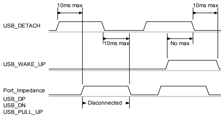
Figure 10.16: USB_DETACH and USB_WAKE_UP Signal
