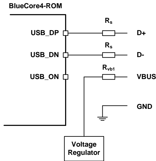
Figure 10.15: USB Connections for Bus Powered Mode
