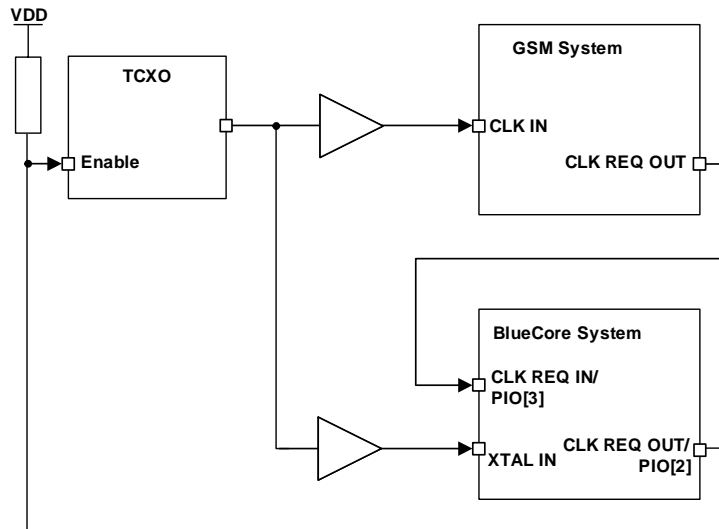
Figure 10.31: Example TXCO Enable OR Function
