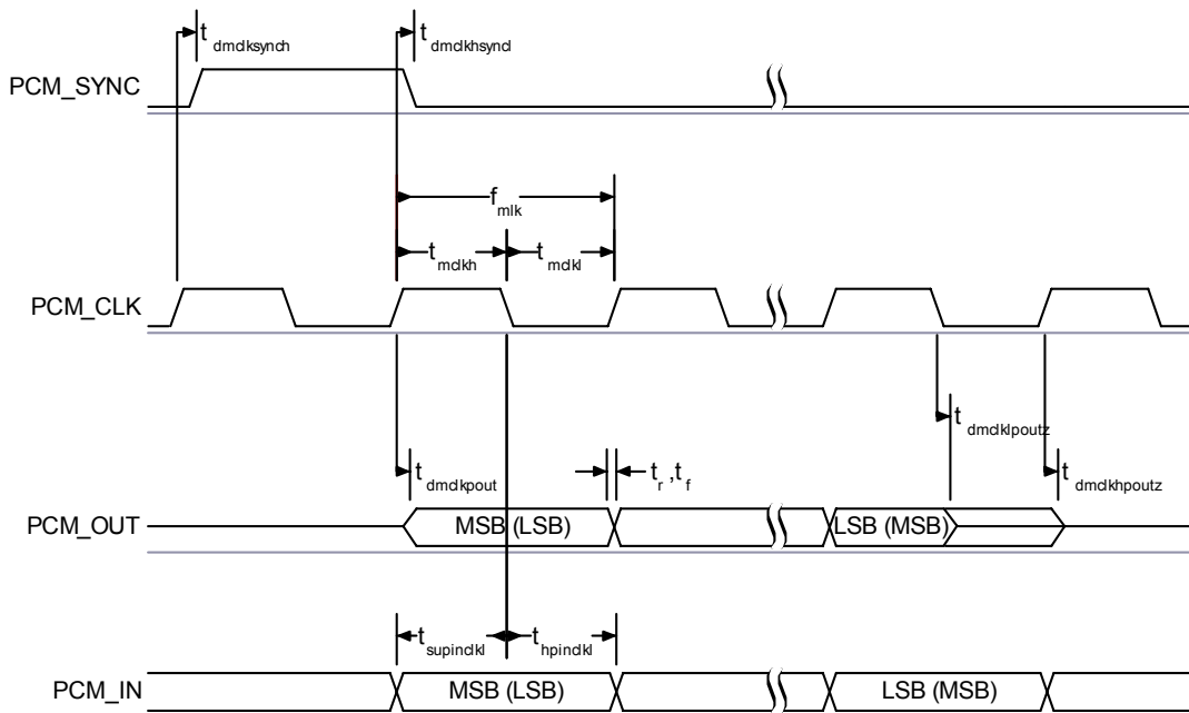
Figure 10.26: PCM Master Timing Long Frame Sync
