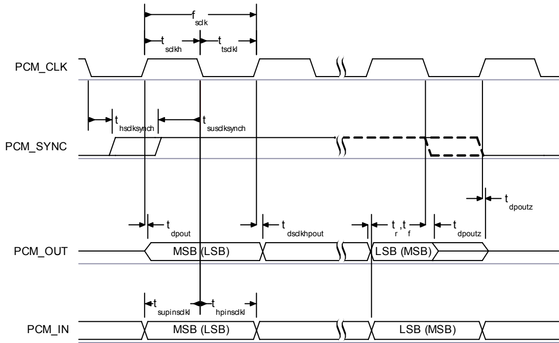
Figure 10.28: PCM Slave Timing Long Frame Sync
