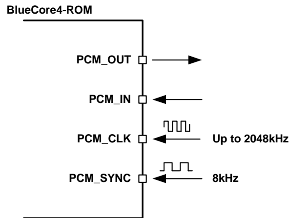
Figure 10.20: BlueCore4-ROM as PCM Interface Slave
