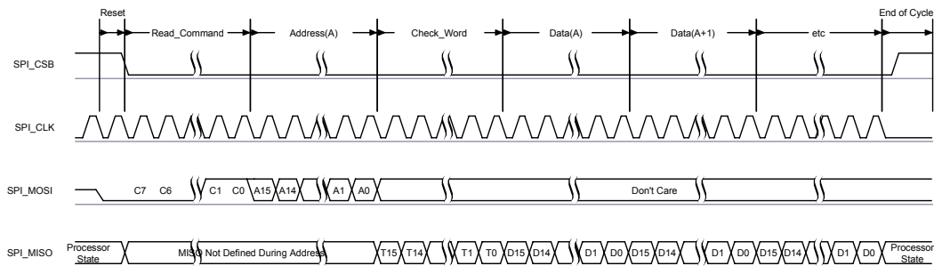
Figure 10.18: Read Operation
