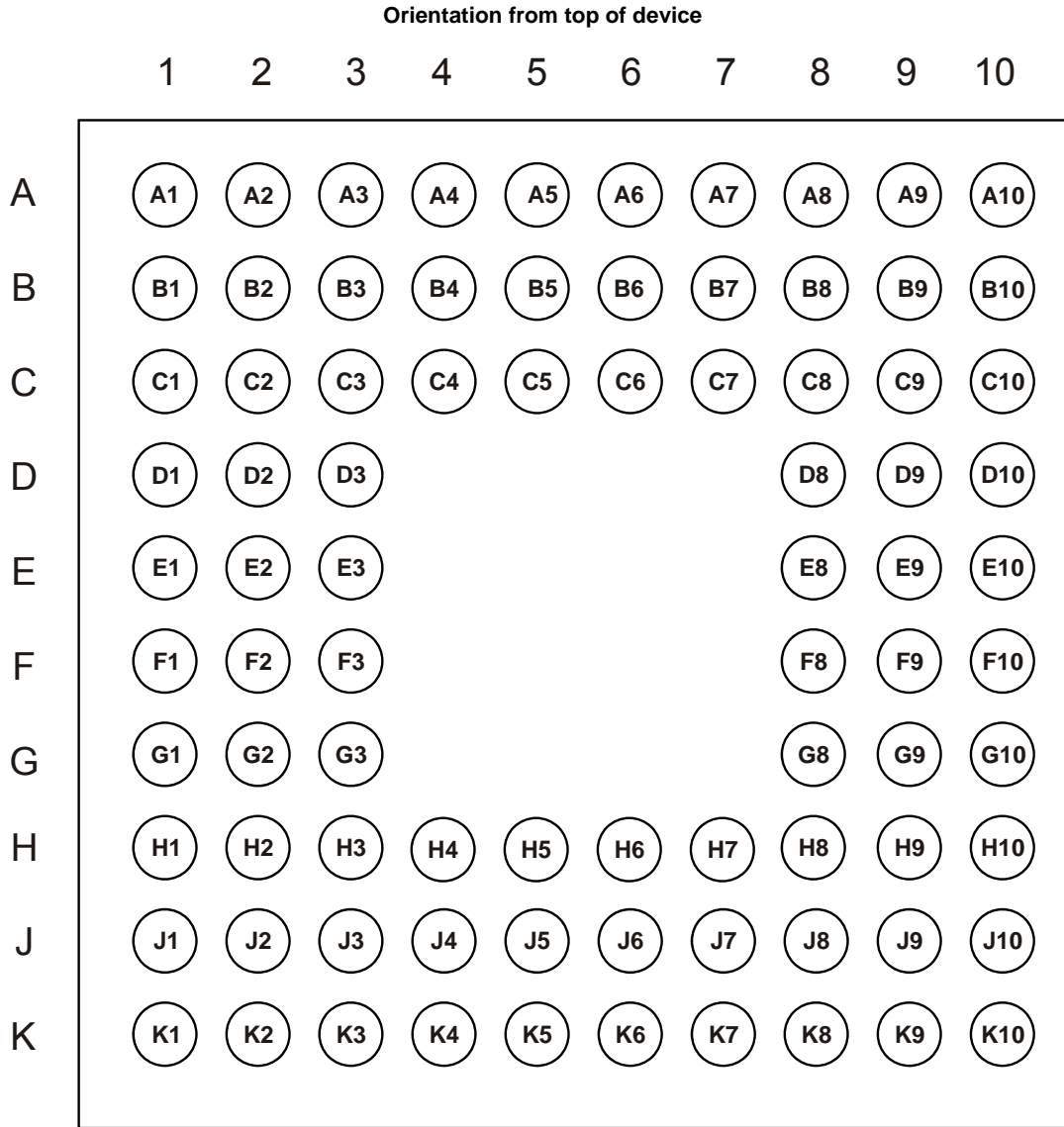
Figure 2.1: BlueCore4-ROM Device Pinout
