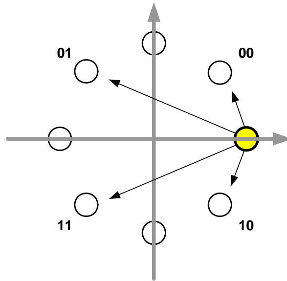
Figure 9.2: \pi/4 DQPSK Constellation Pattern
