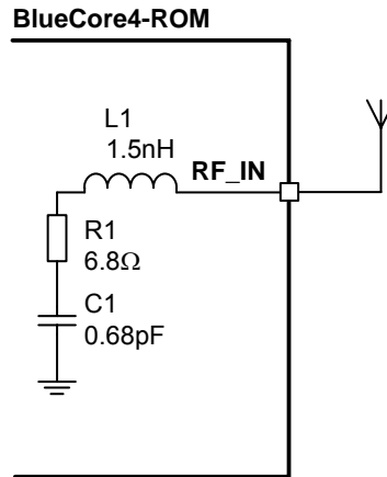
Figure 10.2: Circuit RF_IN
