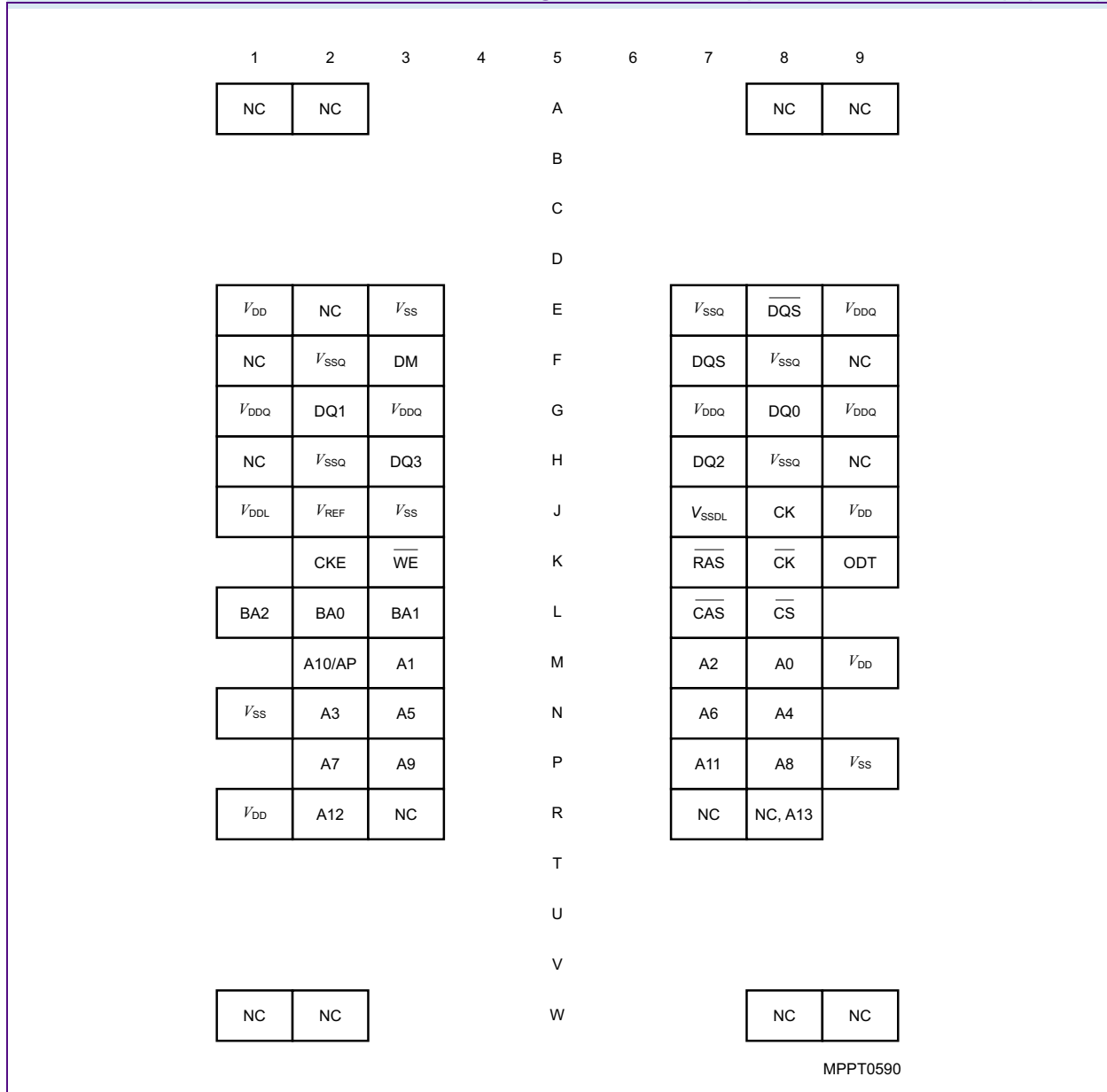
FIGURE 1 Ball Configuration for ×4 components, PG-TFBGA-68 (top view)
