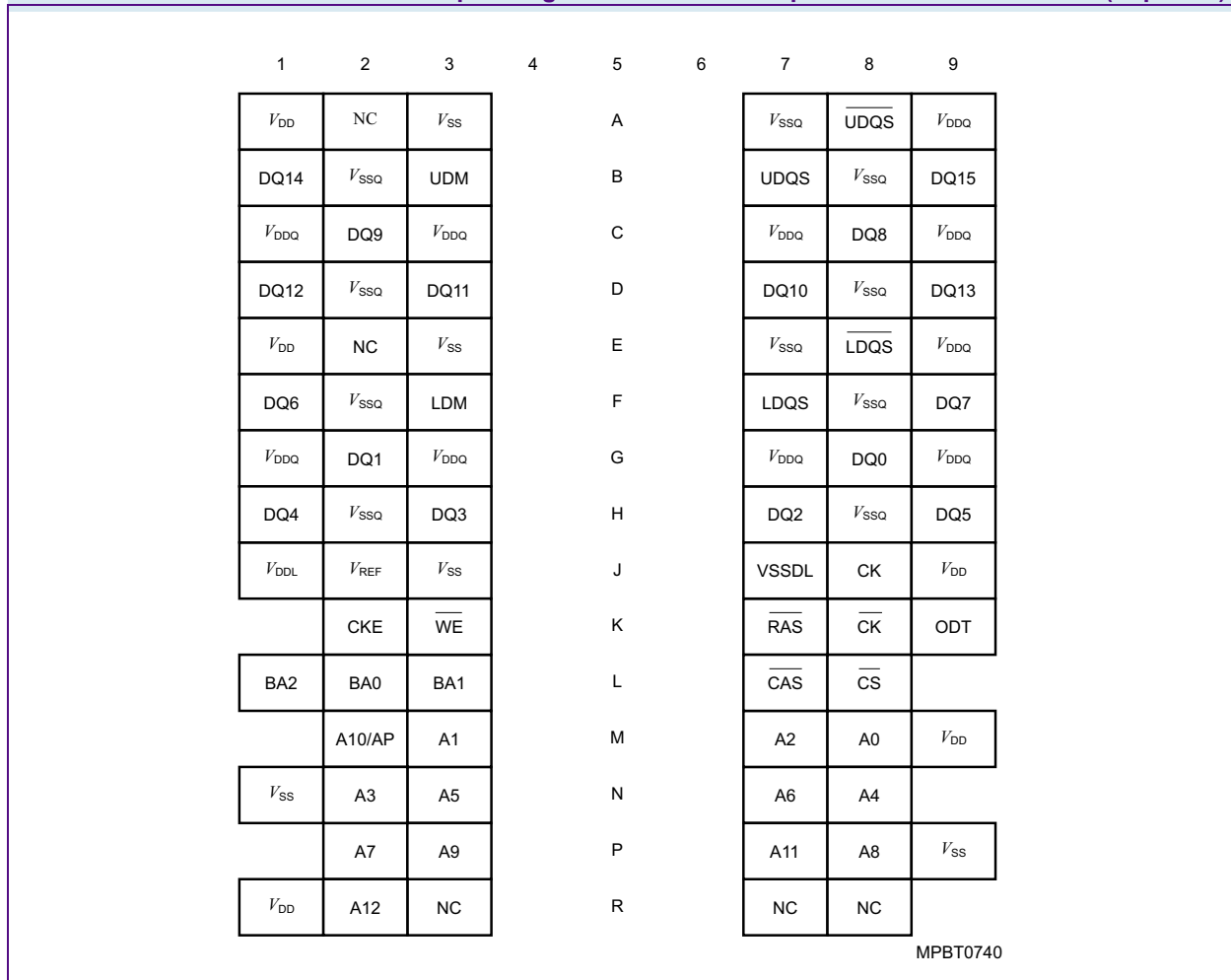
Chip Configuration for x16 Components in PG-TFBGA-84 (Top view)
