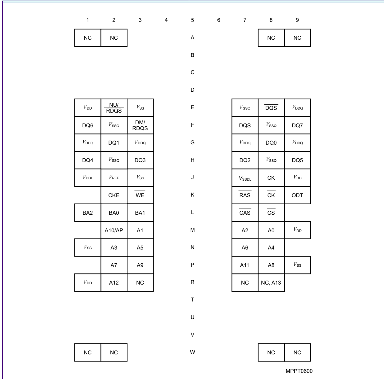
FIGURE 2 Ball Configuration for ×8 components, PG-TFBGA-68 (top view)
