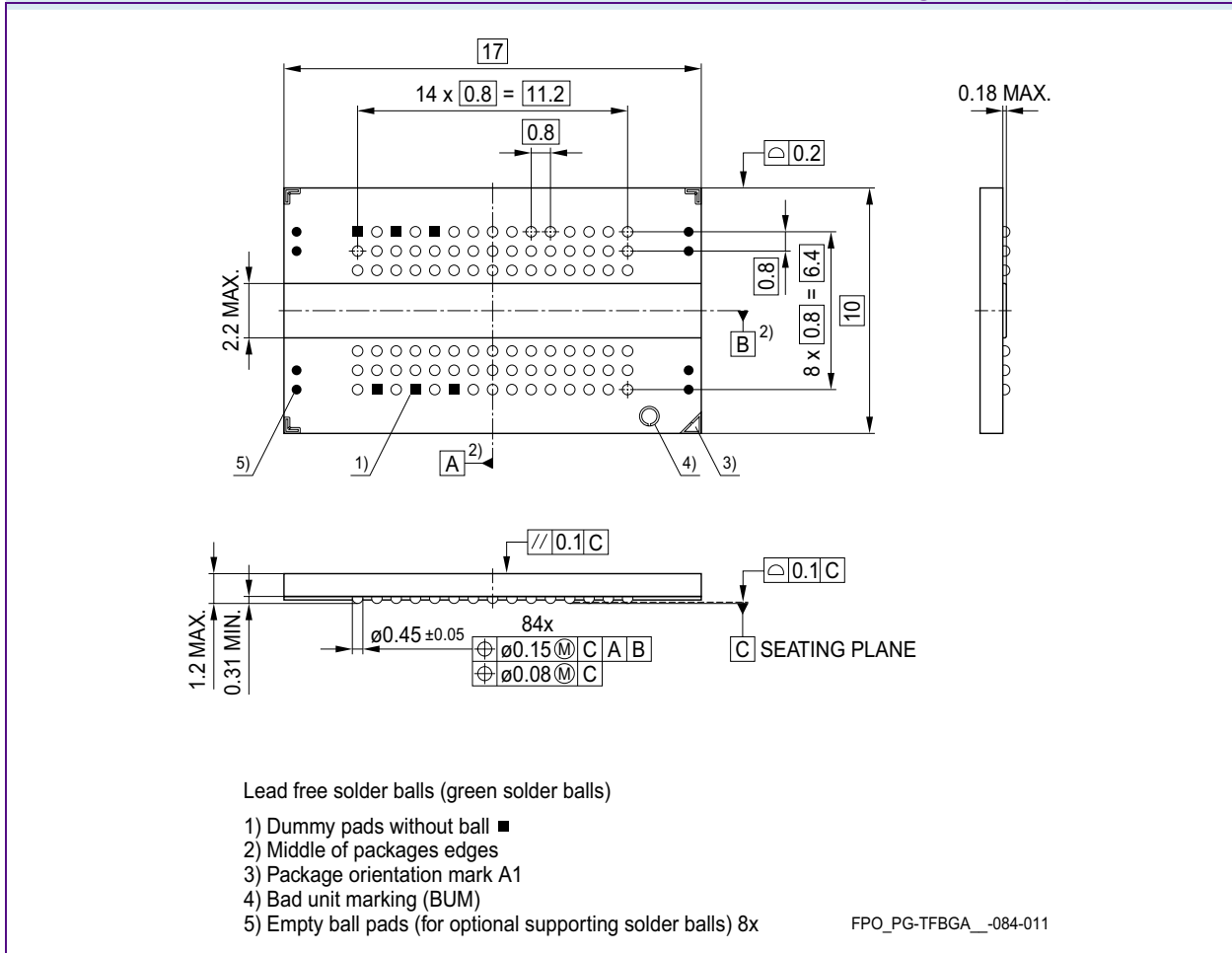
FIGURE 12 Package Outline P(G)-TFBGA-84
