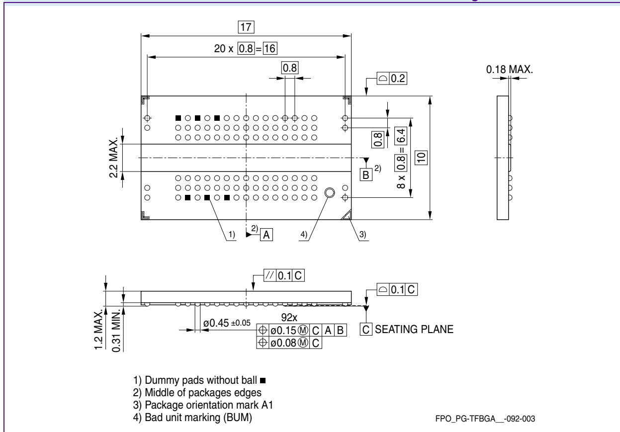
FIGURE 13 Package Outline PG-TFBGA-92
