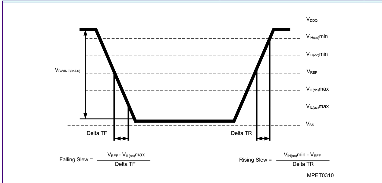
FIGURE 4 Single-ended AC Input Test Conditions Diagram
