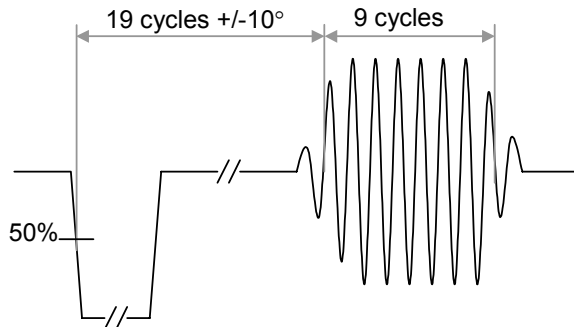
Fig. 16 Synchronizing Signal and Burst Waveform(NTSC)
