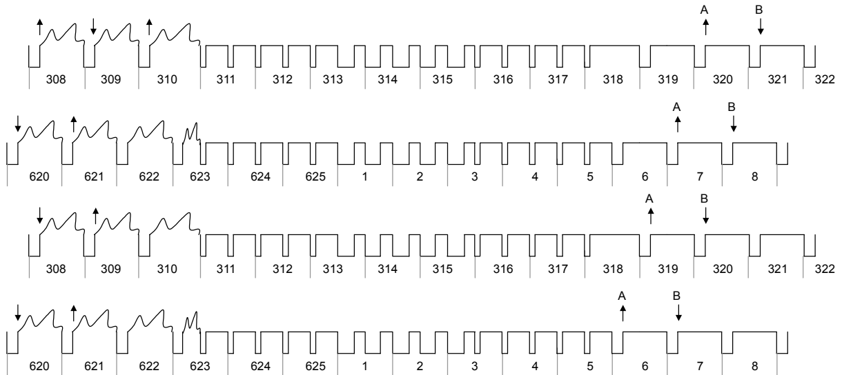
Fig. 21 FID/VSYNC Timing and Phase of Burst
