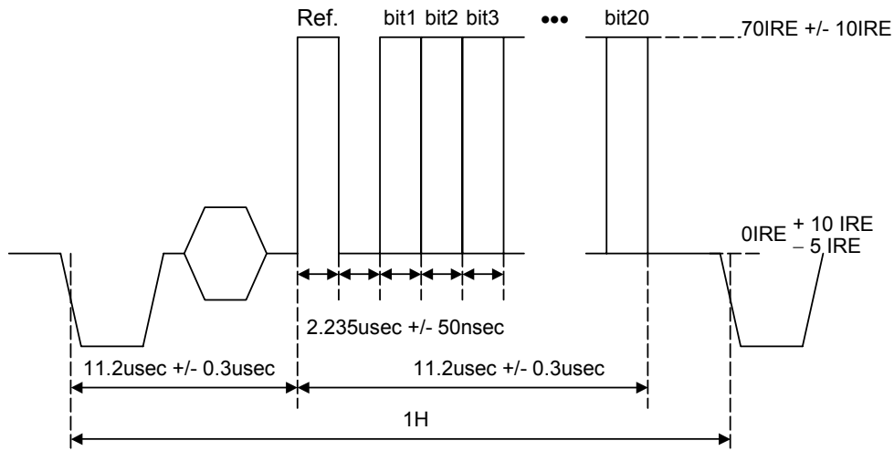
Fig. 7 VBID Wave Form
