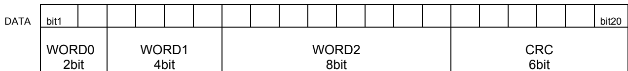
Fig. 6 VBID code assignment
