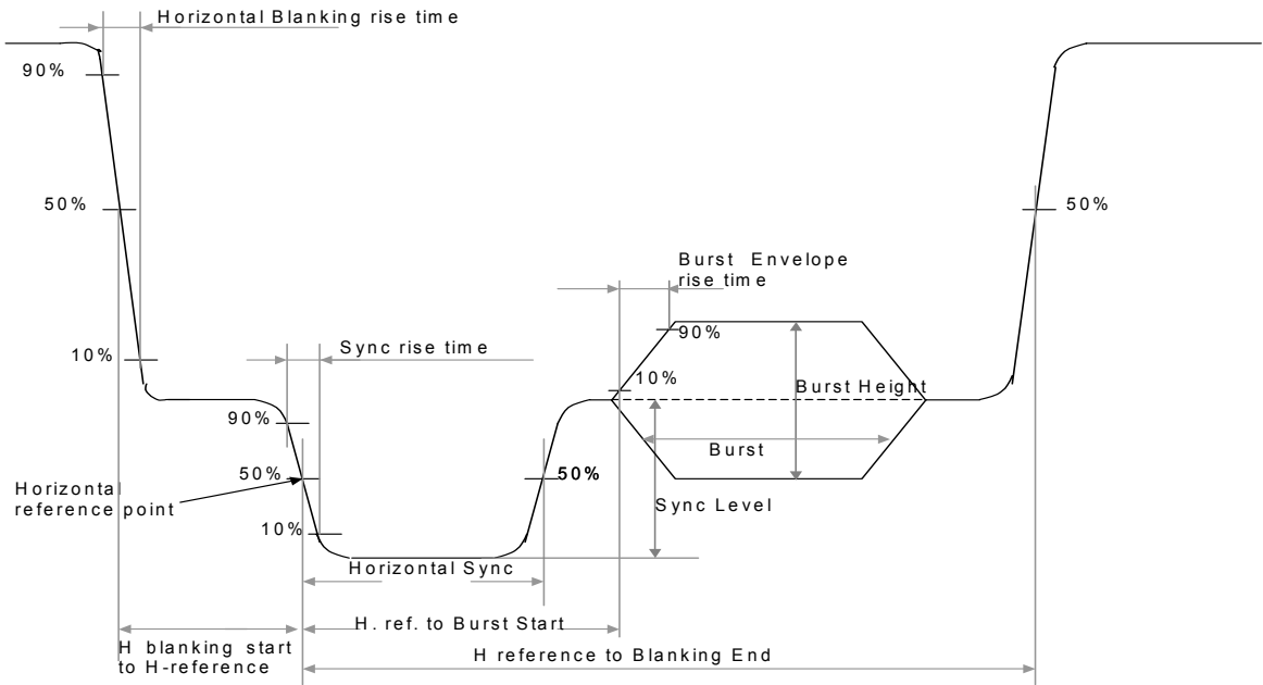
Fig. 20 PAL Waveform
