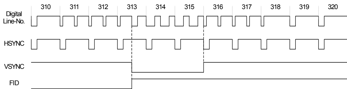
Fig. 13 HSYNC FID/VSYNC Timing
