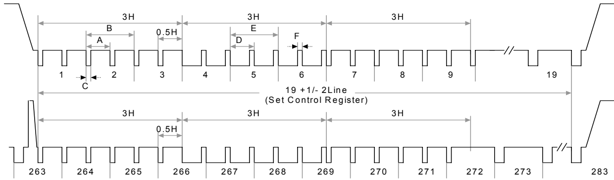
Fig. 17 HSYNC Timing
