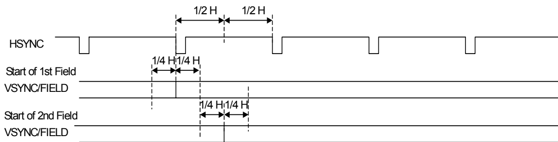
Fig. 12 Video Field
