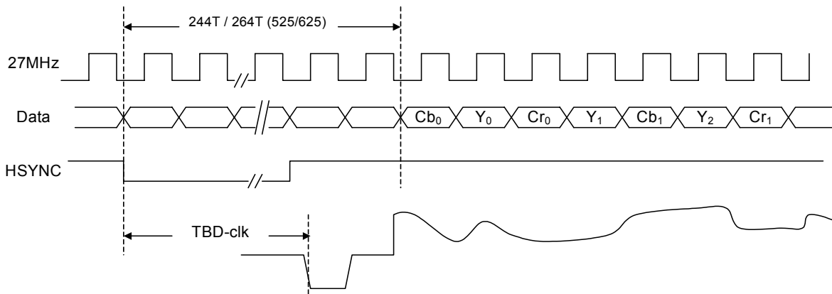
Fig. 11 Interfacing timing (Slave mode)
