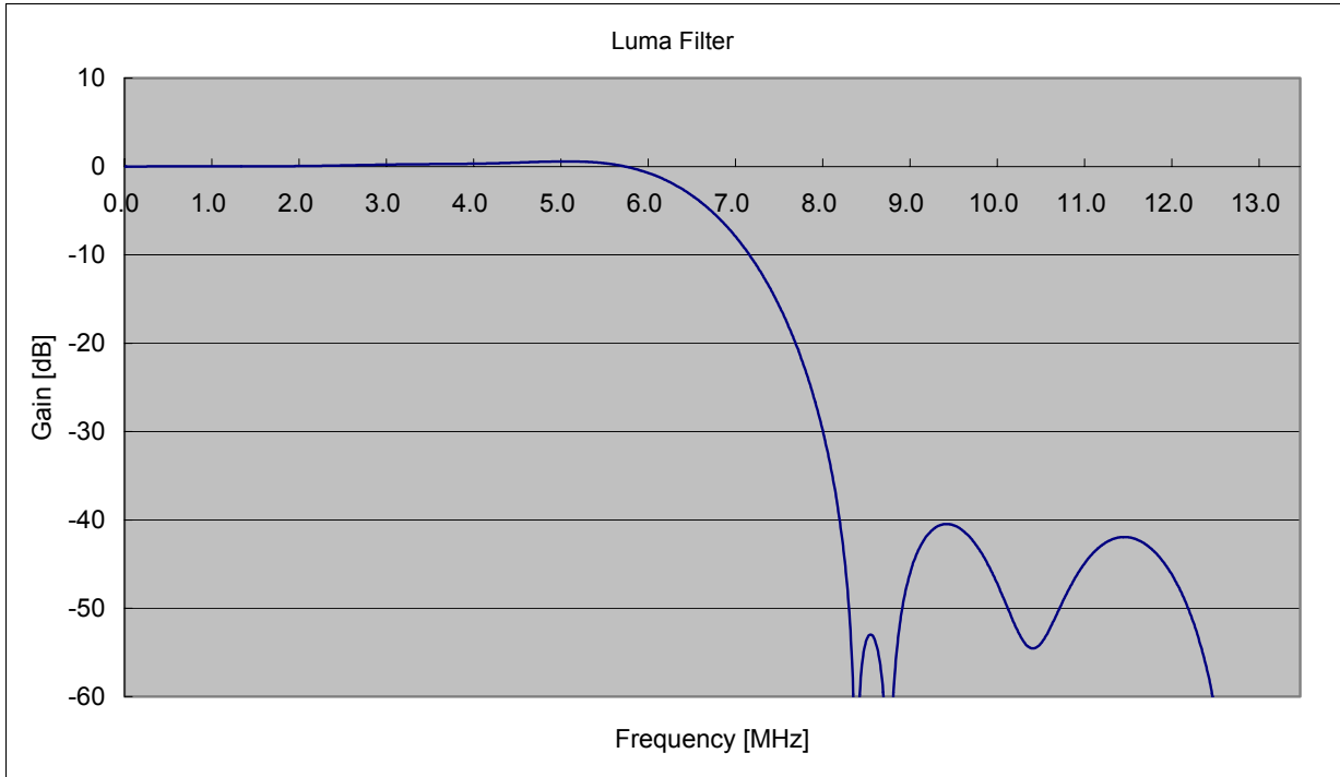
Fig. 1 Luminance Filter
