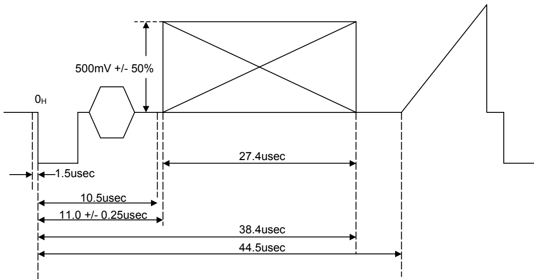
Fig. 8 WSS Data Renewal Timing
