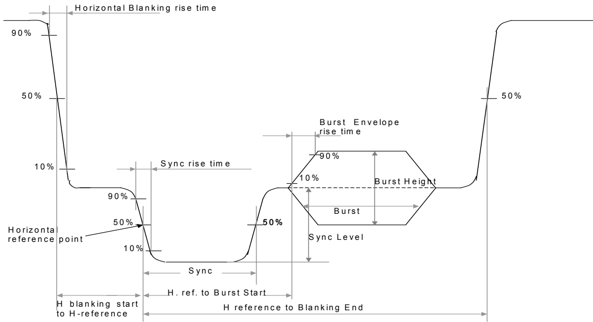
Fig. 15 Synchronizing Signal and Burst Waveform
