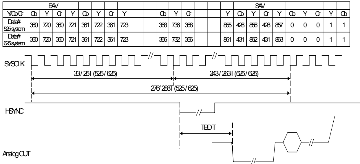
Fig. 10 Interface Timing (ITU-R BT.656 or Master mode)
