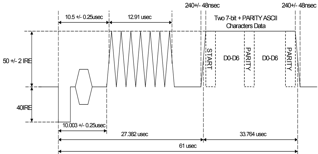
Fig. 4 Closed Captioning Wave form
