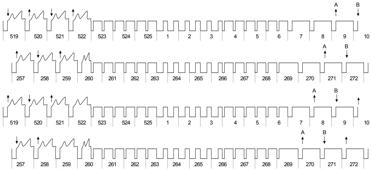
Fig. 19 FID/VSYNC Timing and Phase of Burst
