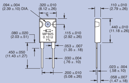
Figure 2 TO-126 Style MP825
