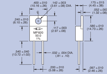
Figure 1 Metal Tab TO-220 Style MP820 and MP821
