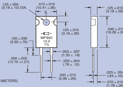
Figure 3 TO-220 Style MP850
