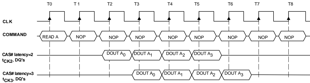
Burst Read Operation (Burst Length = 4, CAS# Latency = 2, 3)
