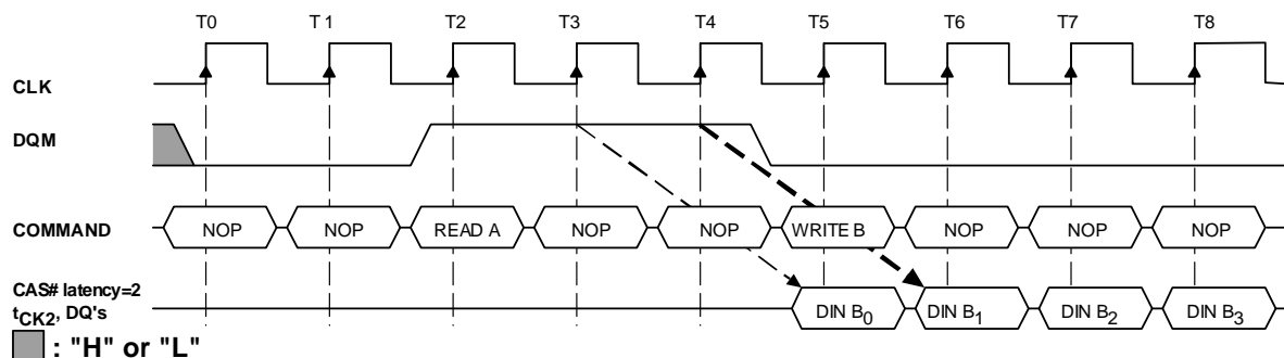
Read to Write Interval (Burst Length 3, CAS# Latency = 2)
