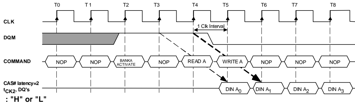
Read to Write Interval (Burst Length 3, CAS# Latency = 2)
