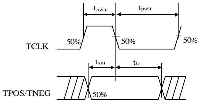
Fig.2 Transmitter Timing
