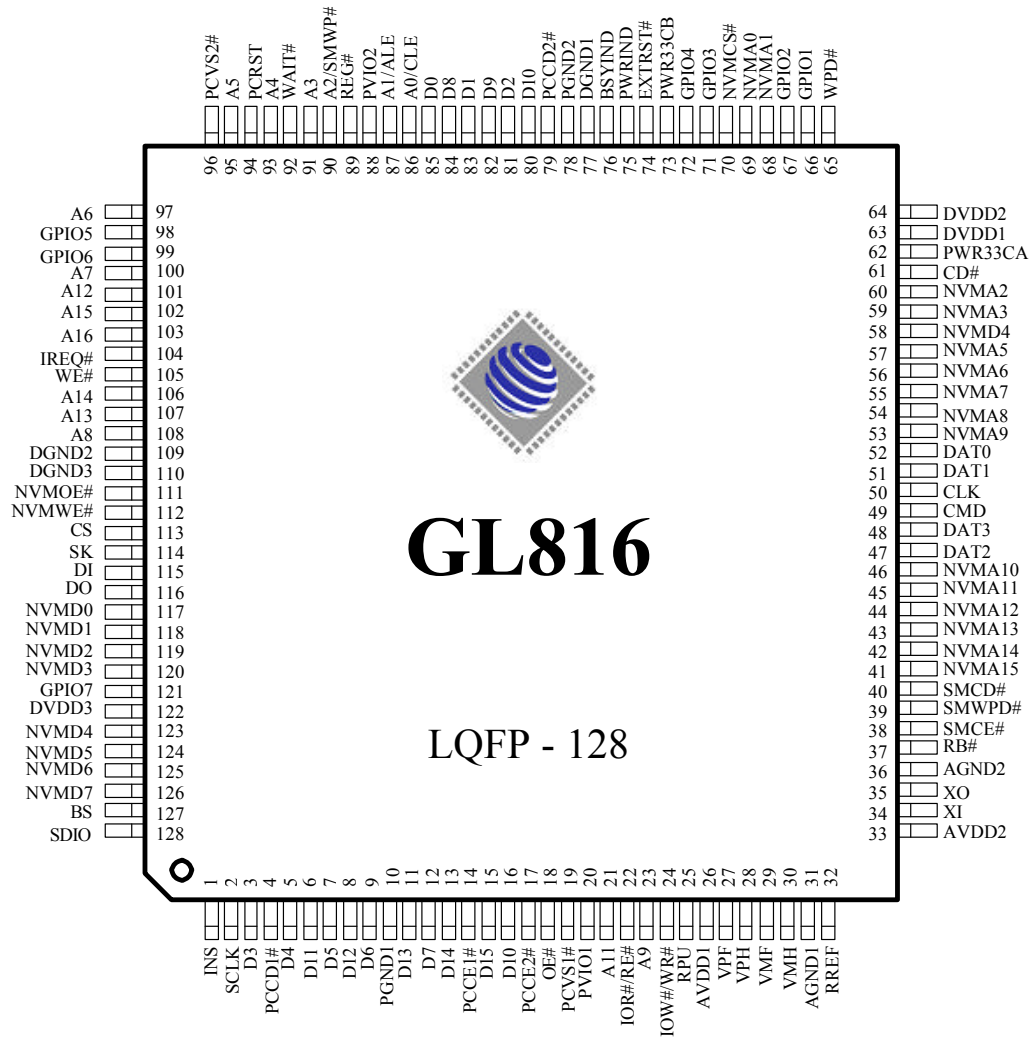
Figure 4.1 - Pinout Diagram
