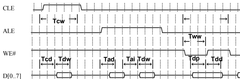
Figure 6.3 - Timing Diagram of SmartMedia
