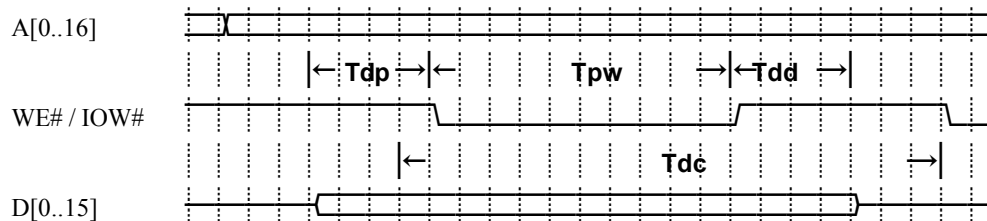
Figure 6.2 - Timing Diagram of PCMCIA
