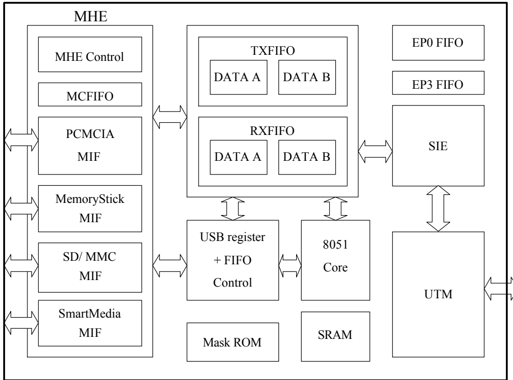
Figure 3.1 - Block Diagram
