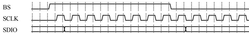
Figure 6.4 - Timing Diagram of MemoryStick
