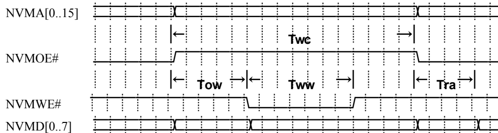
Figure 6.1 - Timing Diagram of External Flash
