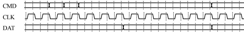
Figure 6.5 - Timing Diagram of SD / MMC Interface
