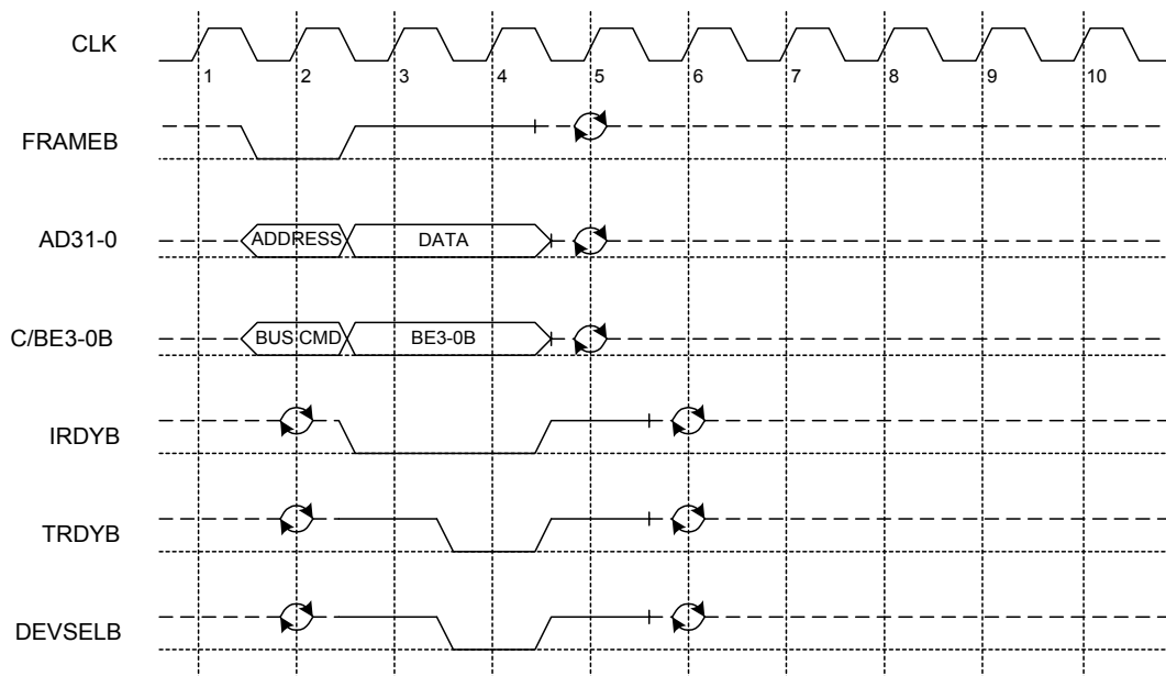
Figure 18. I/O Write
