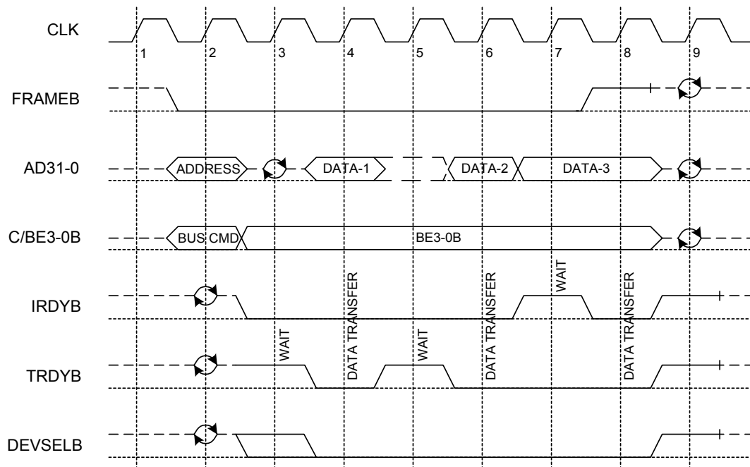
Figure 22. Memory Read Below 4GB
