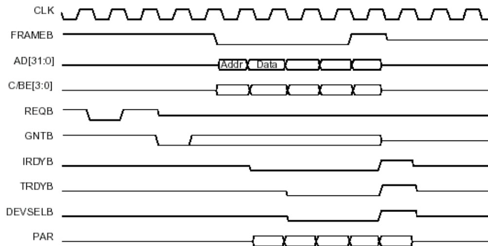
Figure 7. Master Write Operation
