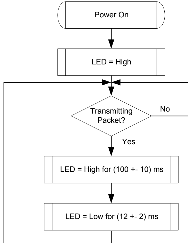
Figure 9. Tx LED
