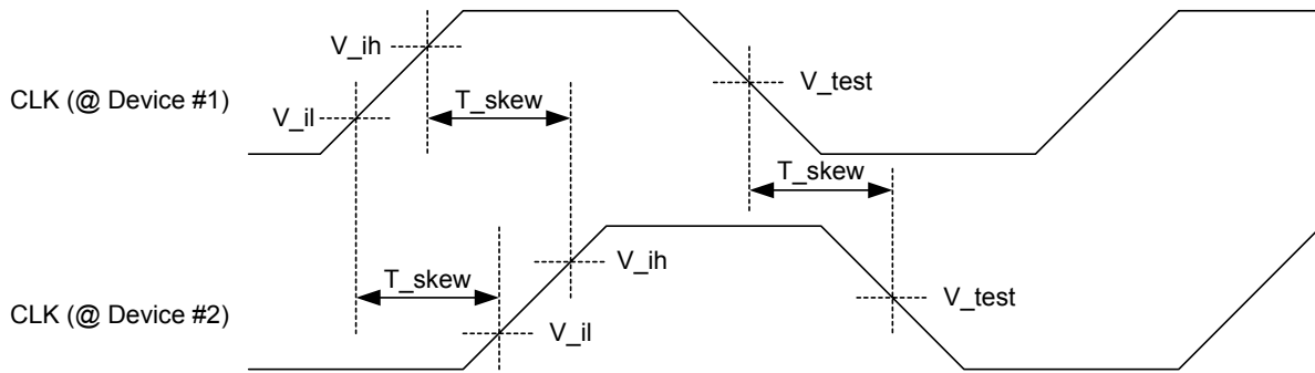
Figure 16. Clock Skew Diagram
