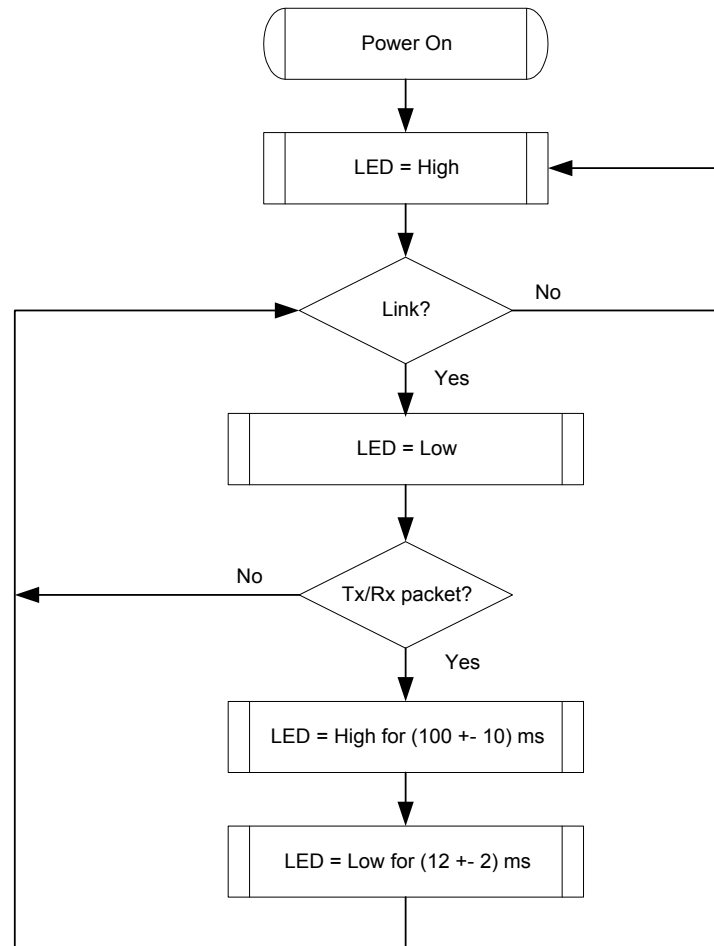
Figure 11. LINK/ACT LED
