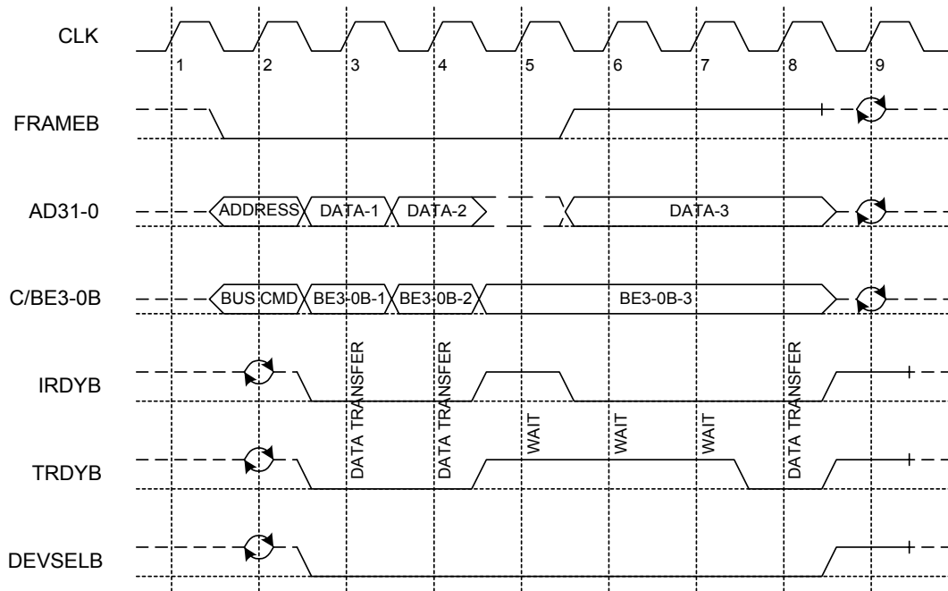
Figure 23. Memory Write Below 4GB
