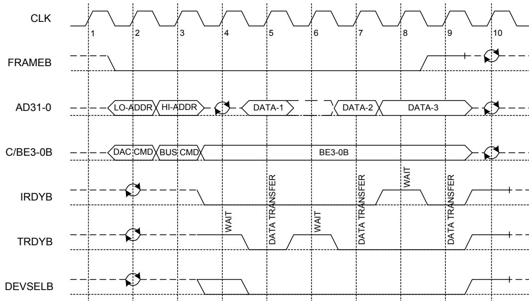
Figure 28. Memory Read Above 4GB (DAC)
