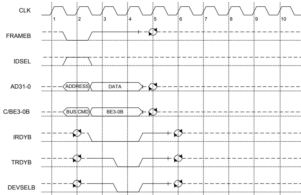
Figure 20. Configuration Write
