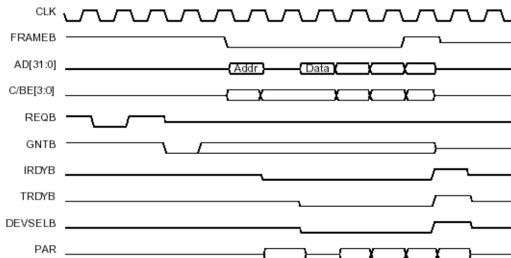
Figure 6. Master Read Operation
