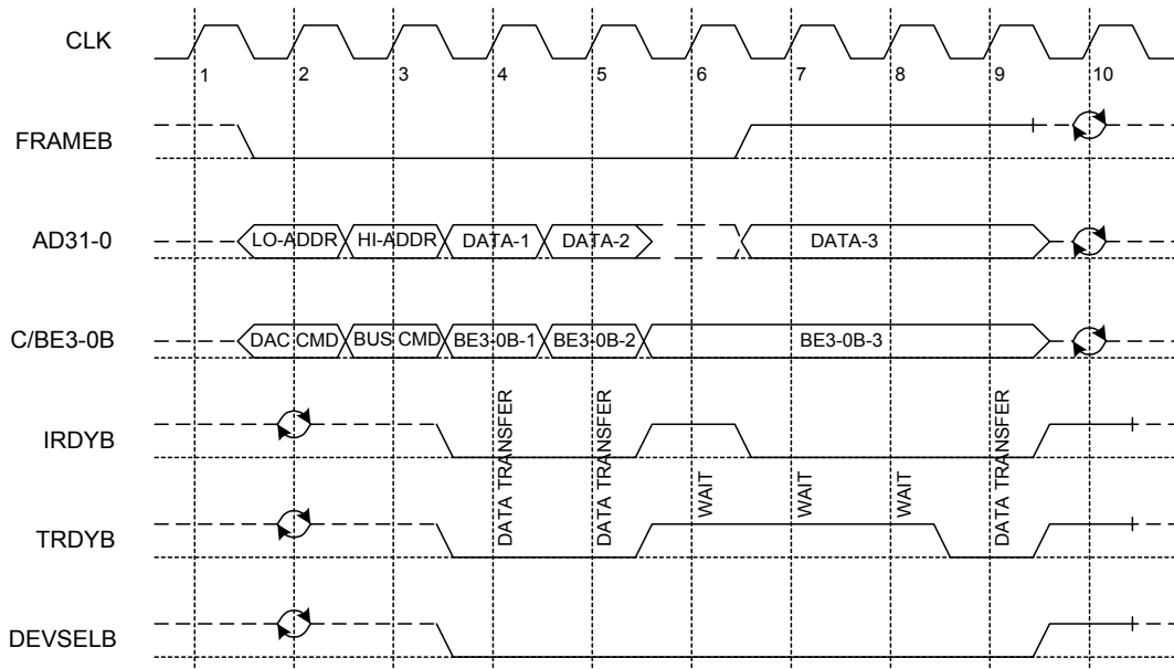
Figure 29. Memory Write Above 4GB (DAC)
