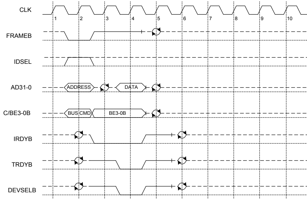
Figure 19. Configuration Read
