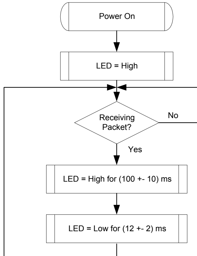
Figure 8. Rx LED
