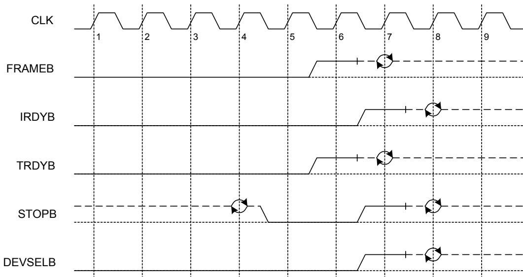
Figure 24. Target Initiated Termination - Disconnect
