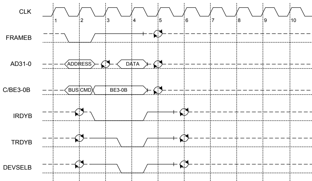
Figure 17. I/O Read
