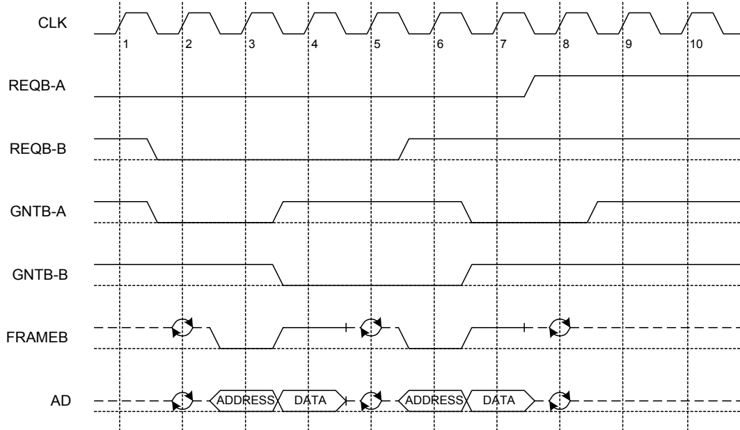
Figure 21. Bus Arbitration
