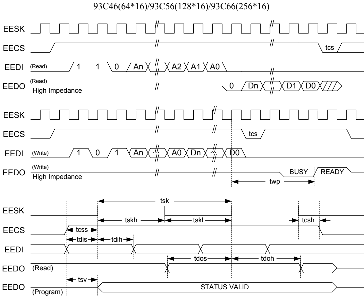
Figure 12. Serial EEPROM Interface Timing
