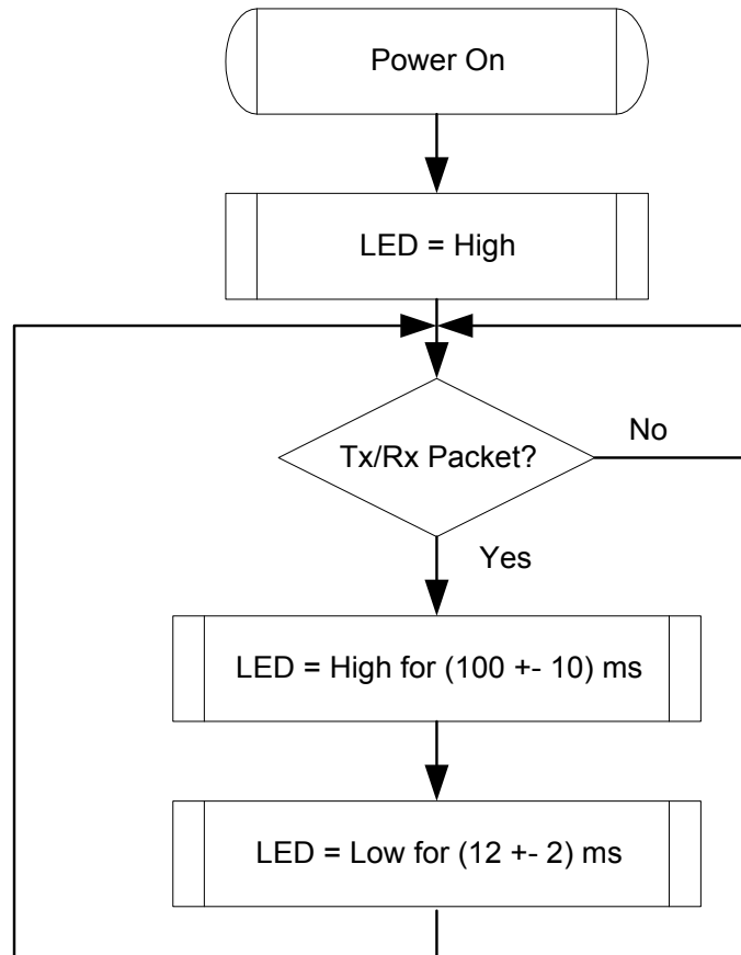
Figure 10. Tx/Rx LED
