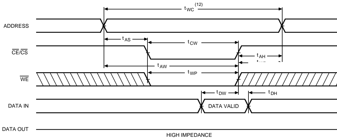
P4C168 (P4C169)
