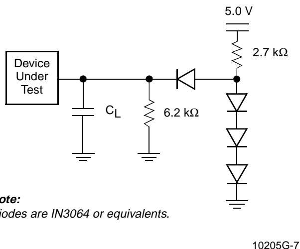
Figure 3. Test Setup
