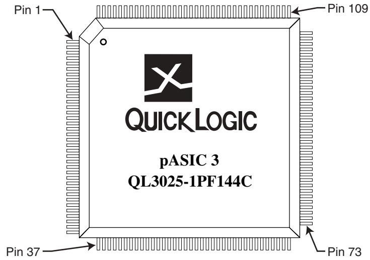
Figure 20: QL3025 – 144 Pin TQFP (Top View)
