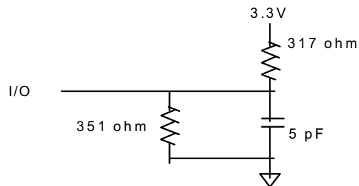
Fig.2 Output Load Equivalent
