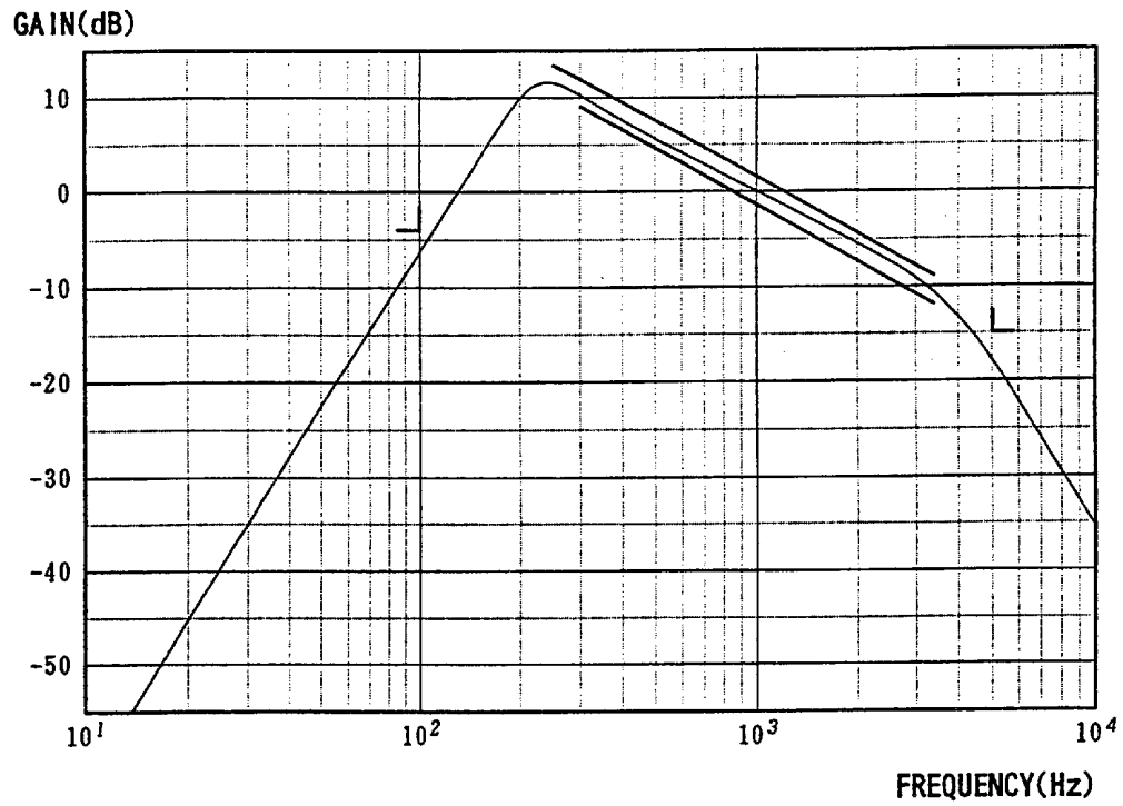
Fig.3 Total Frequency Response of Receiver Section
