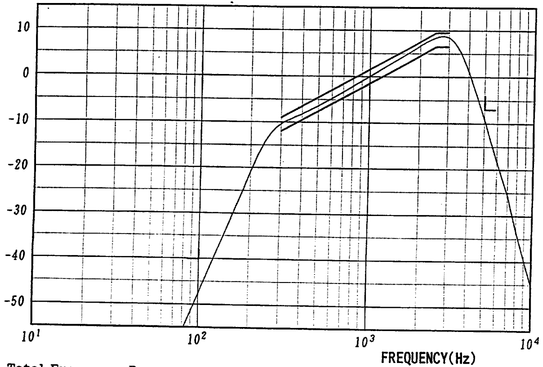
Fig.2 Total Frequency Response of Transmitter Section (FCONT="L")
