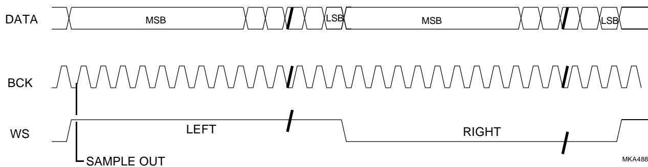
Figure 4-5 Format of Input Signals
