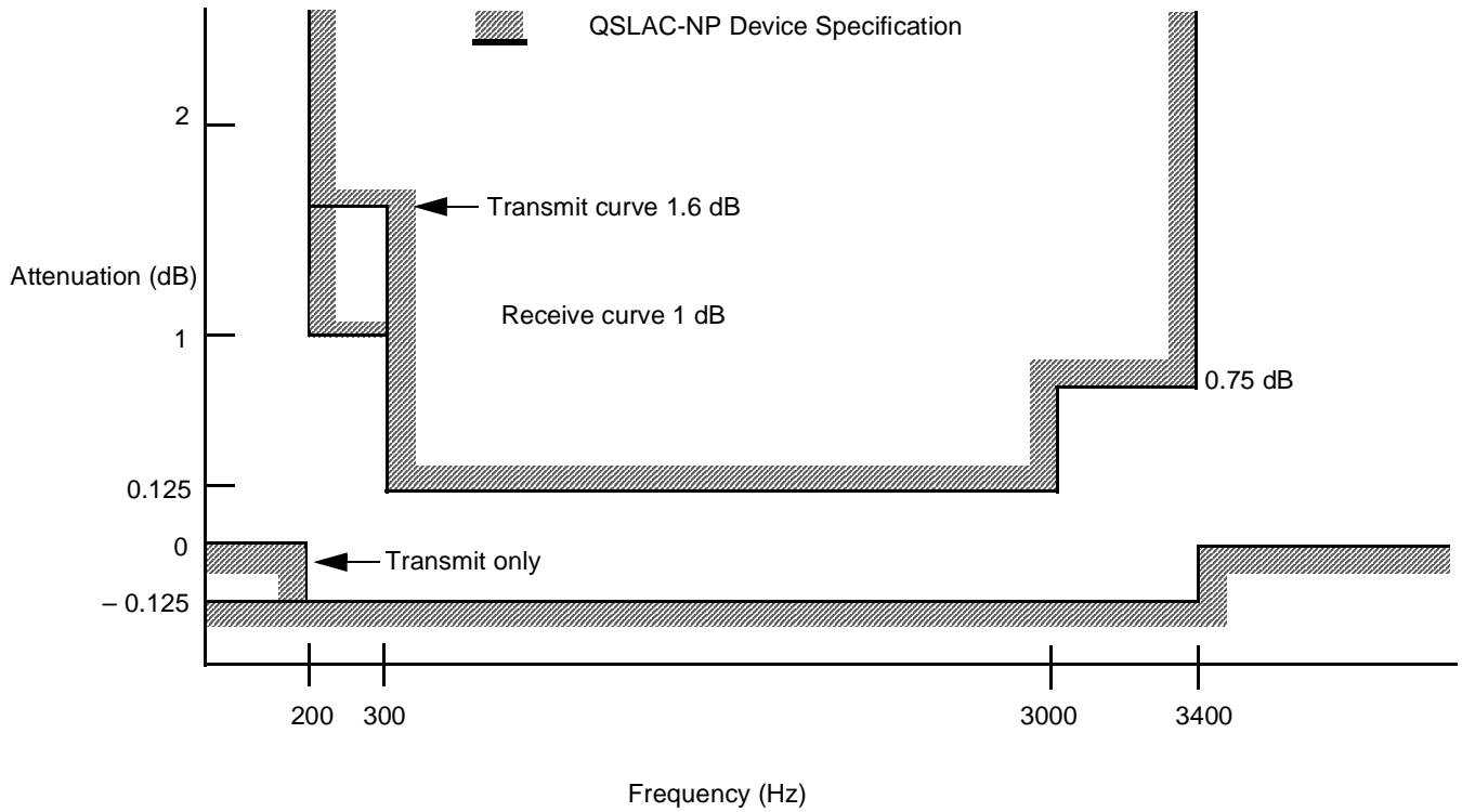
Figure 1. Attenuation Distortion
