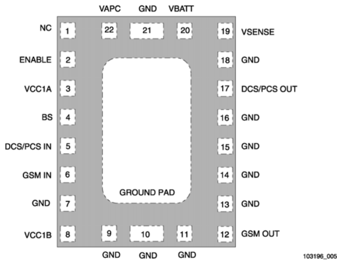
Figure 5. SKY77325 PAM Pin Configuration—22-Pin Leadless (Top View)
