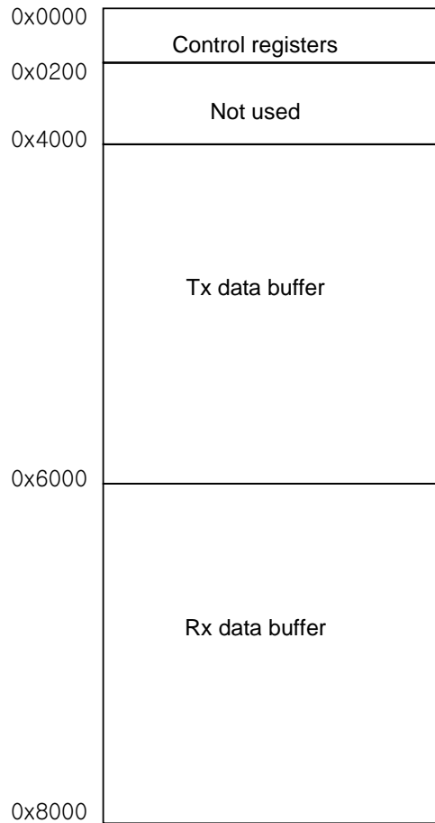
W3100A Top level Memory Map
