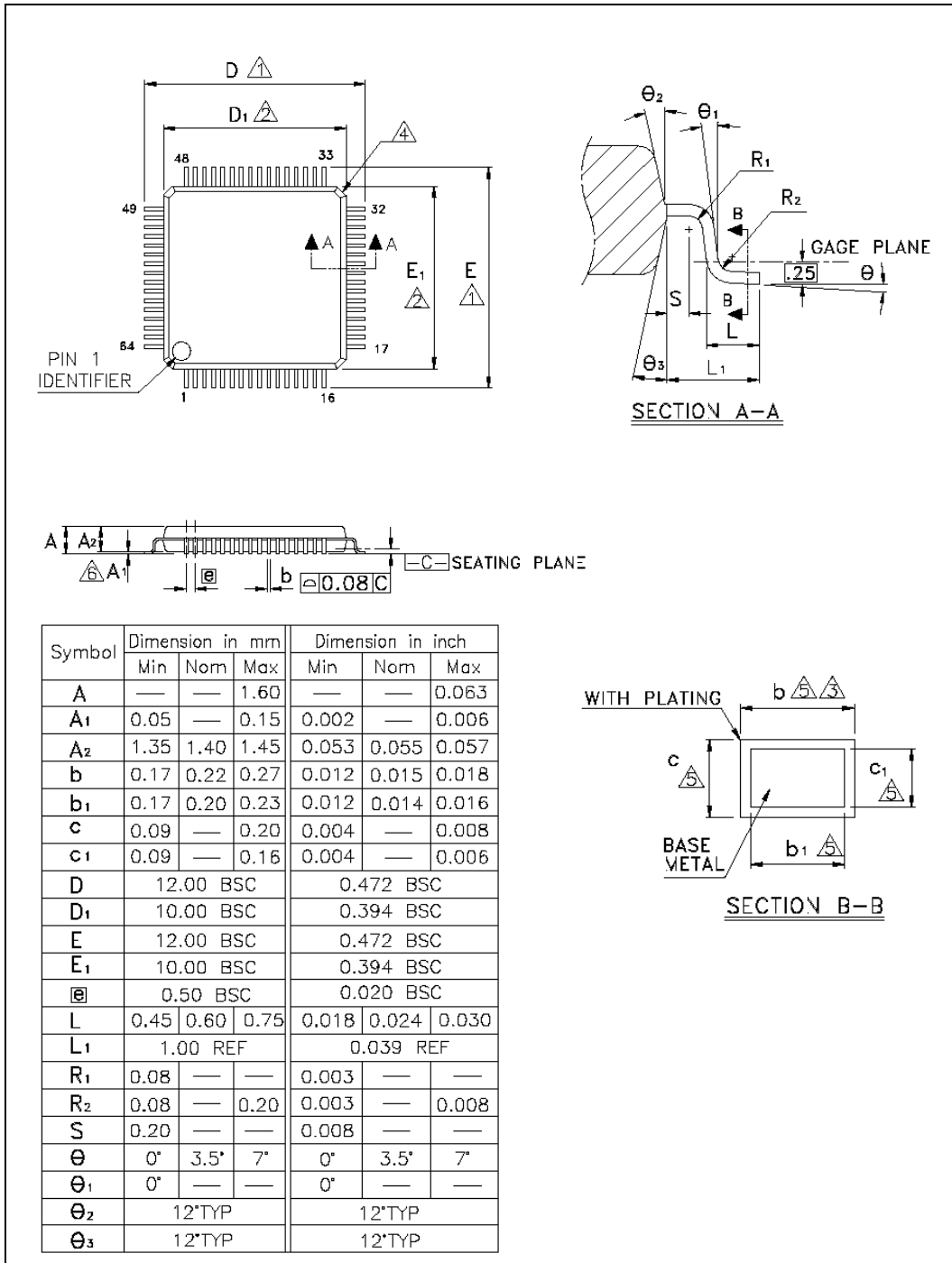
Figure 1: W3100A LQFP Package Specifications
