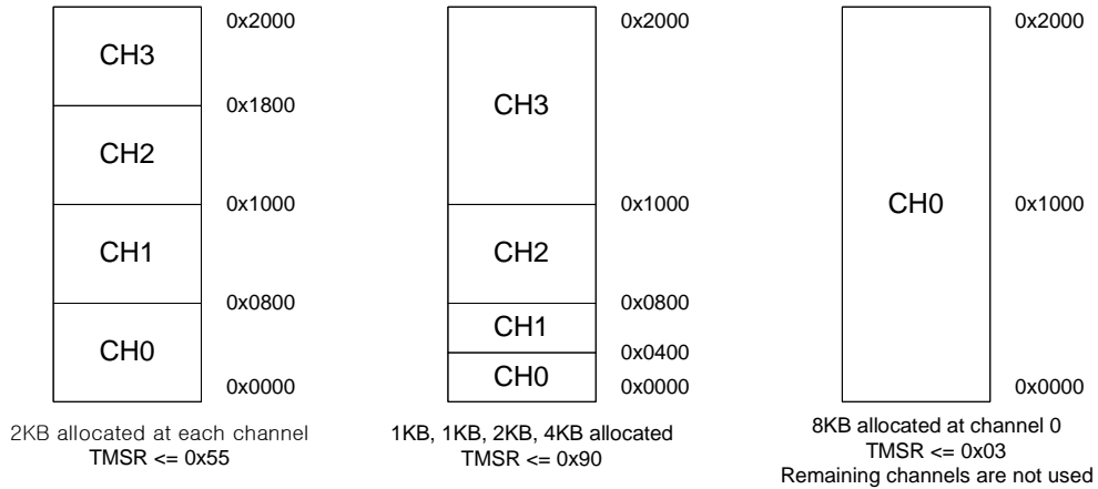
Transmission Memory Allocation
