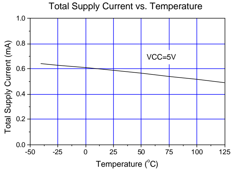
Fig.7 : Total Supply Current vs. Temperature
