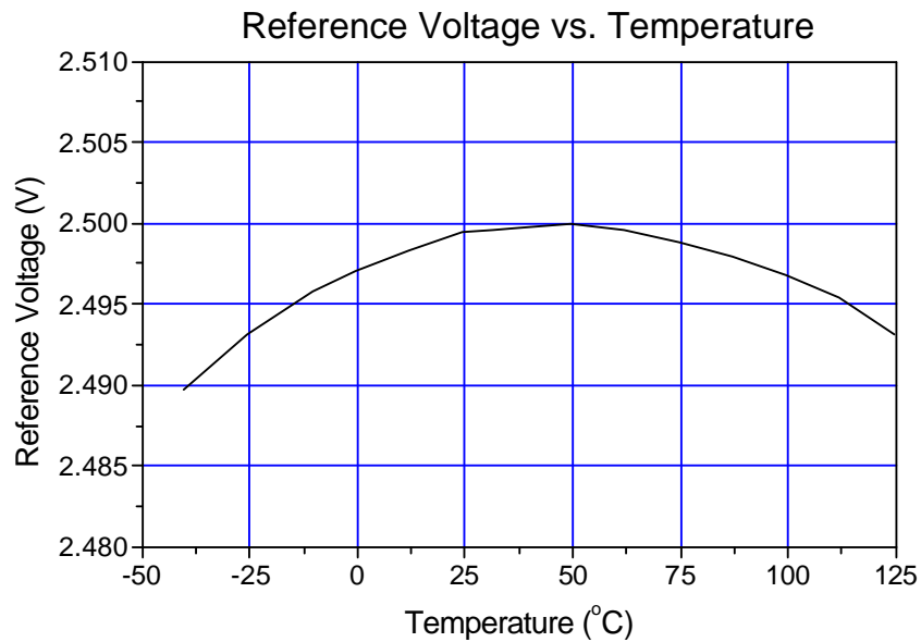
Fig.2 : Reference Voltage vs. Temperature
