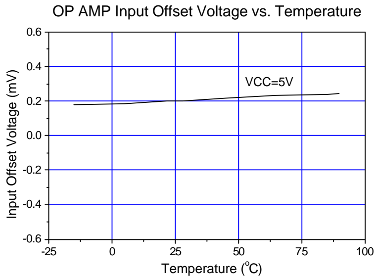
Fig.8 : OP AMP Input Offset Voltage vs. Temperature
