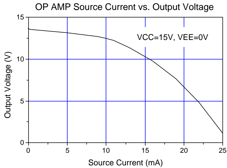
Fig.5 : OP AMP Source Current vs. Output Voltage
