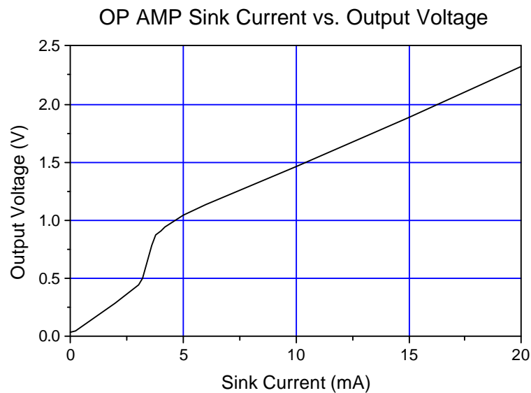
Fig.6 : OP AMP Sink Current vs. Output Voltage
