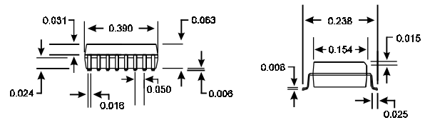
16-Pin SOIC Package
