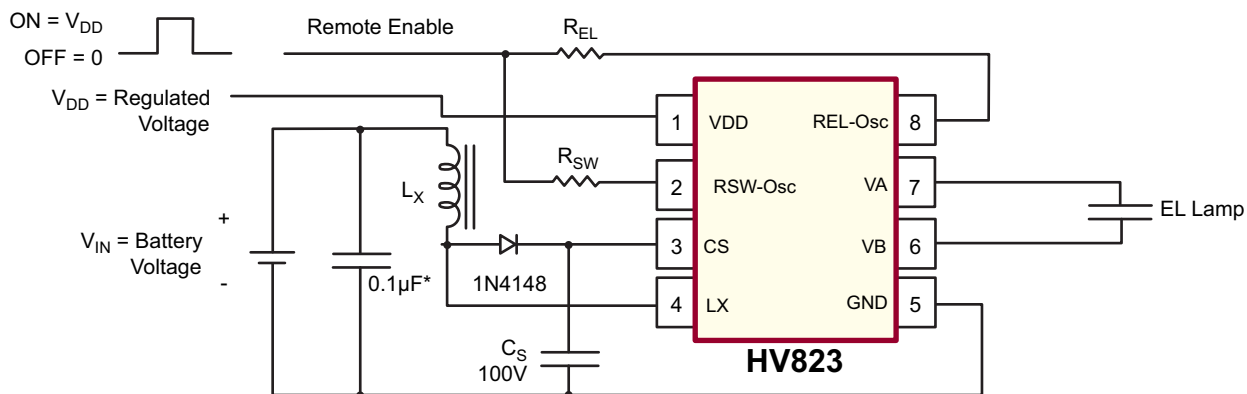
Fig. 5: Split Supply Configuration
