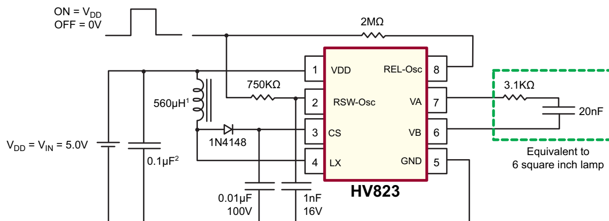
Fig. 2: Typical 5.0V Application
