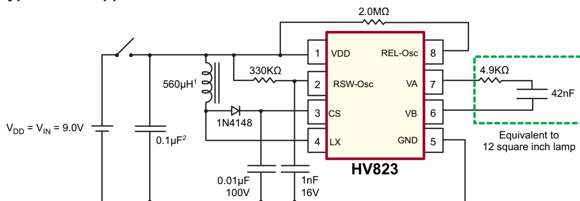
Fig. 3: Typical 9.0V Application
