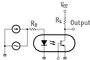
Test Circuit for Frequency Response
