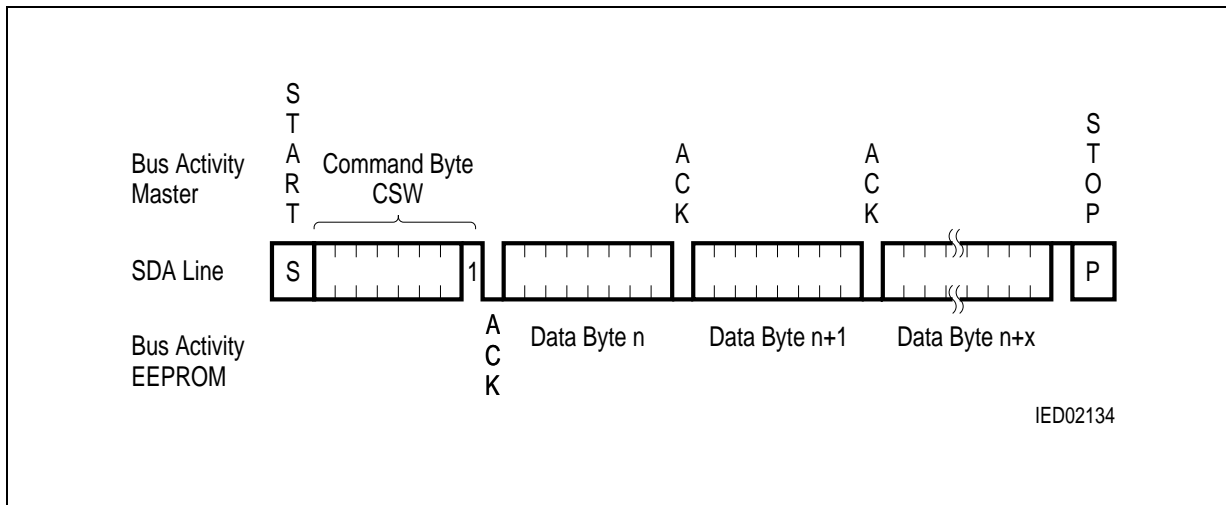
Figure 13 Sequential Read
