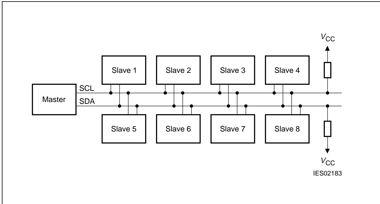
Figure 3 Bus Configuration
