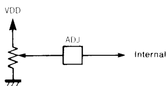
Example of VCO free-run adjustment circuit
