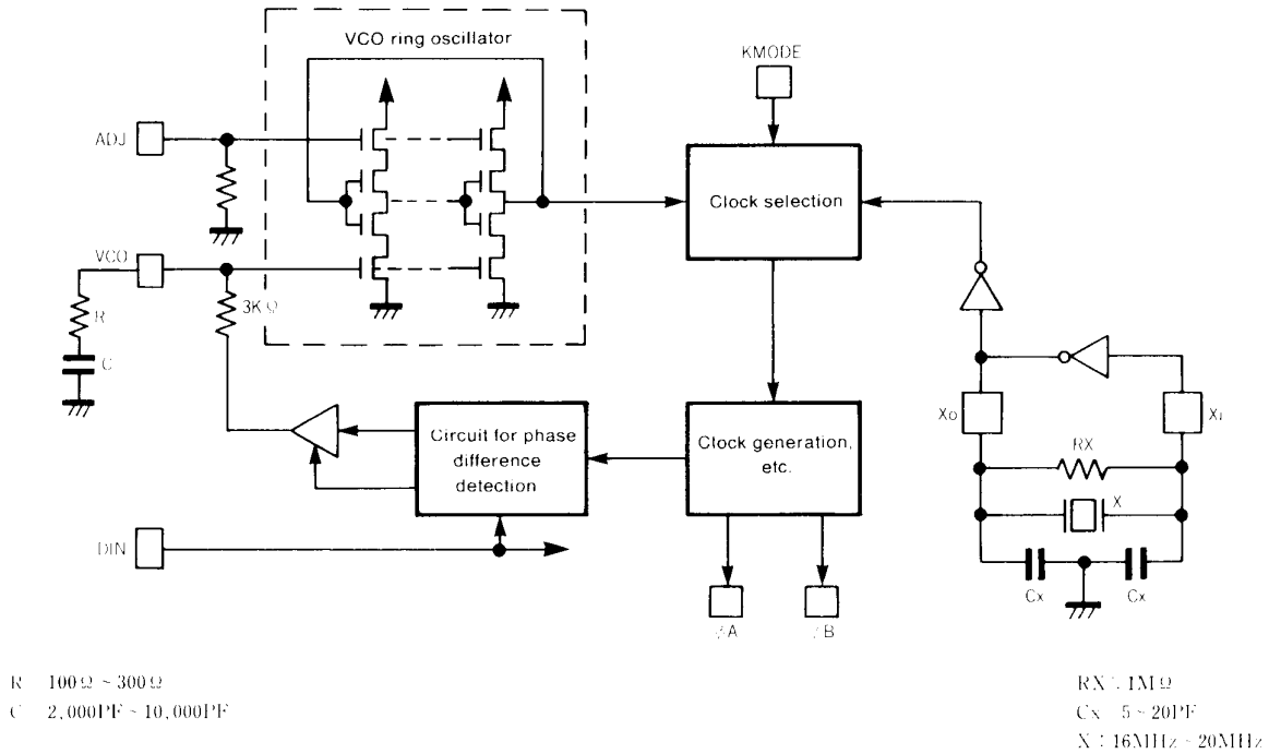
Block diagram of clock circuit
