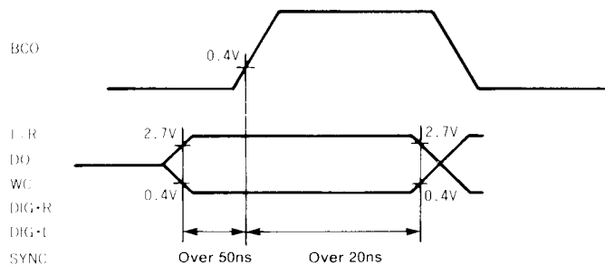
Output timing
